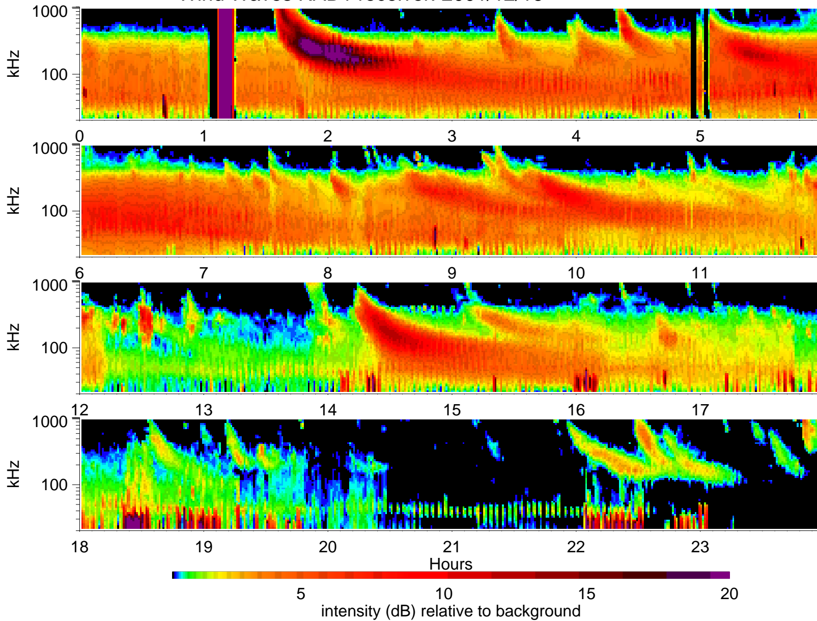
Wind Waves RAD1 receiver: 2001/12/16
