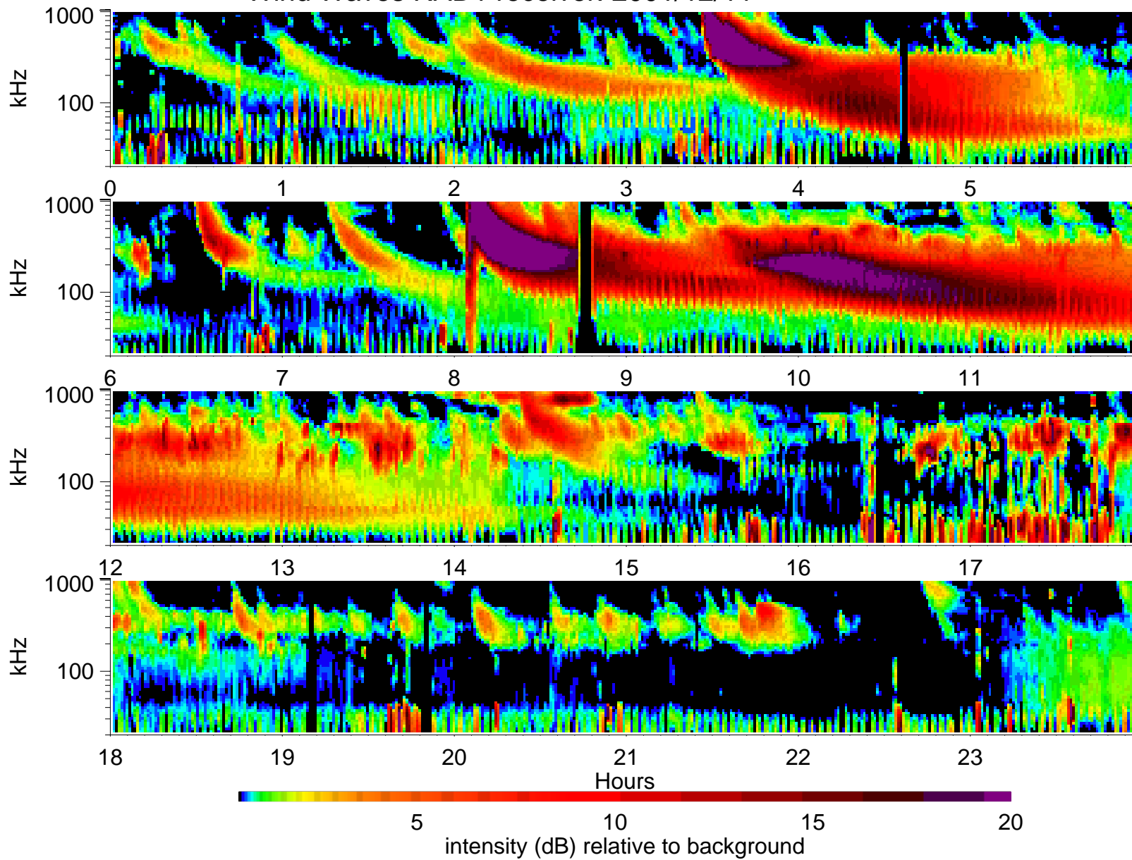
Wind Waves RAD1 receiver: 2001/12/11
