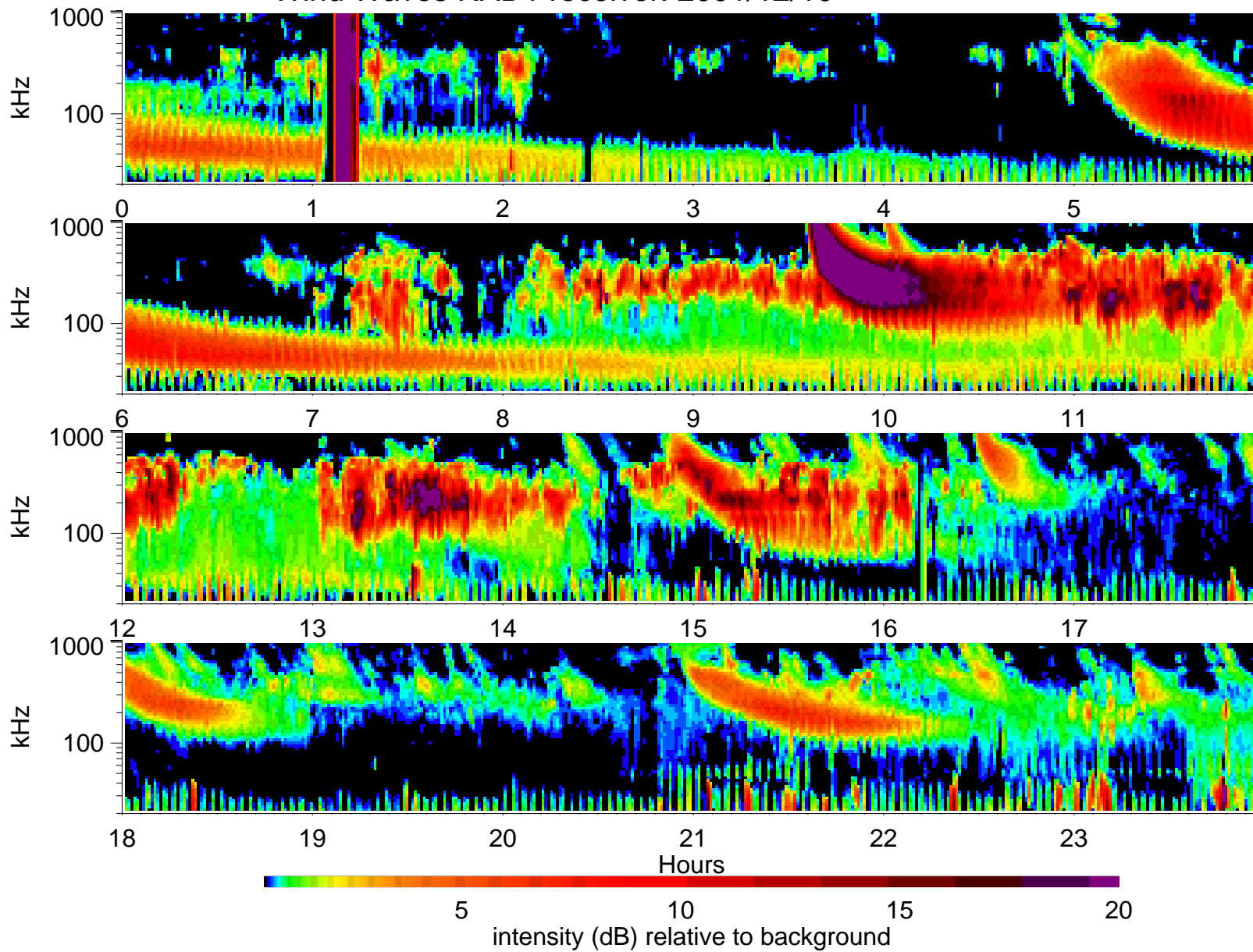
Wind Waves RAD1 receiver: 2001/12/10
