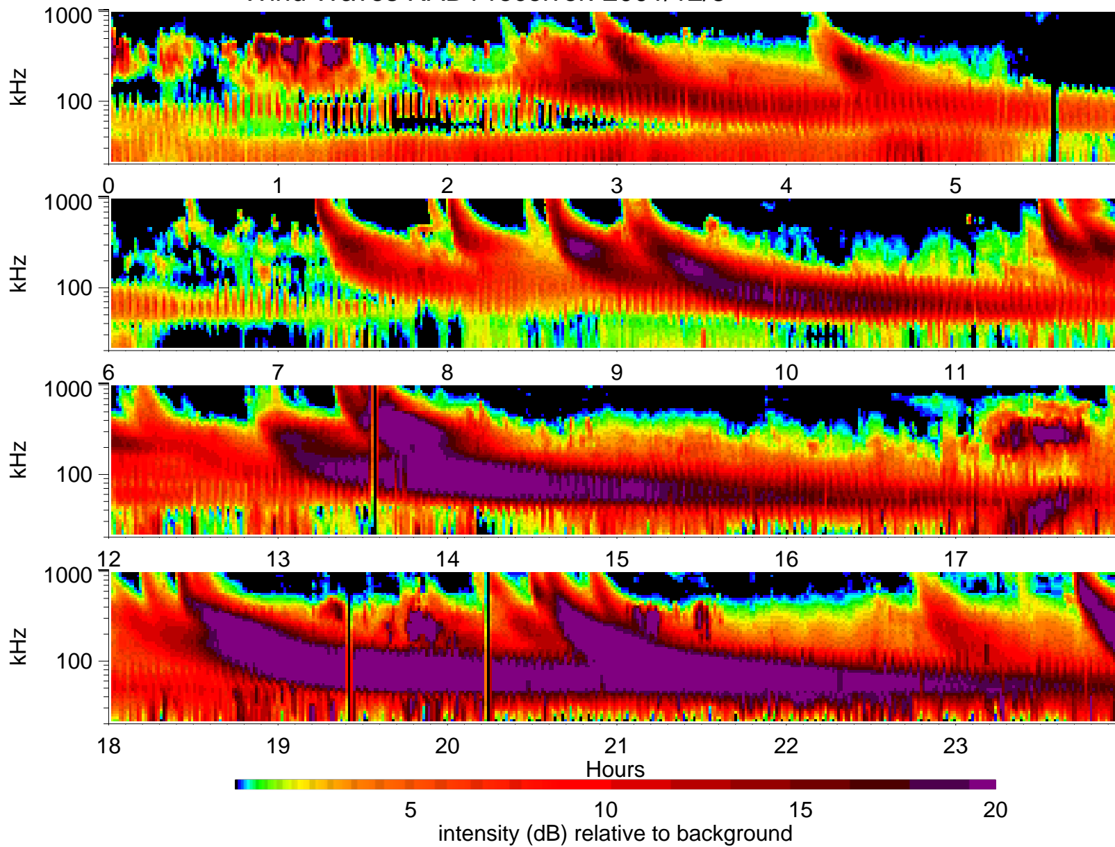
Wind Waves RAD1 receiver: 2001/12/3
