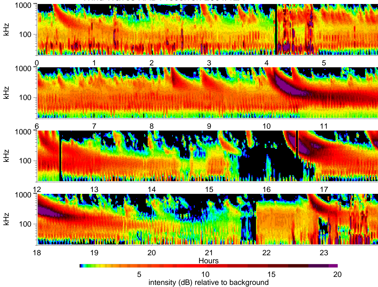
Wind Waves RAD1 receiver: 2001/12/1
