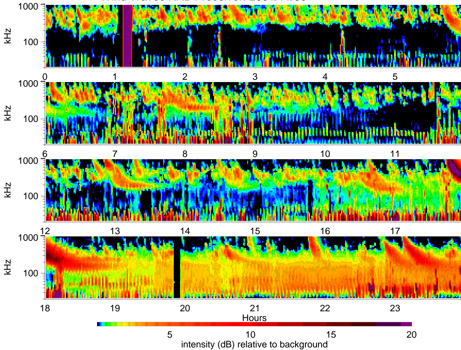
Wind Waves RAD1 receiver: 2001/11/30
