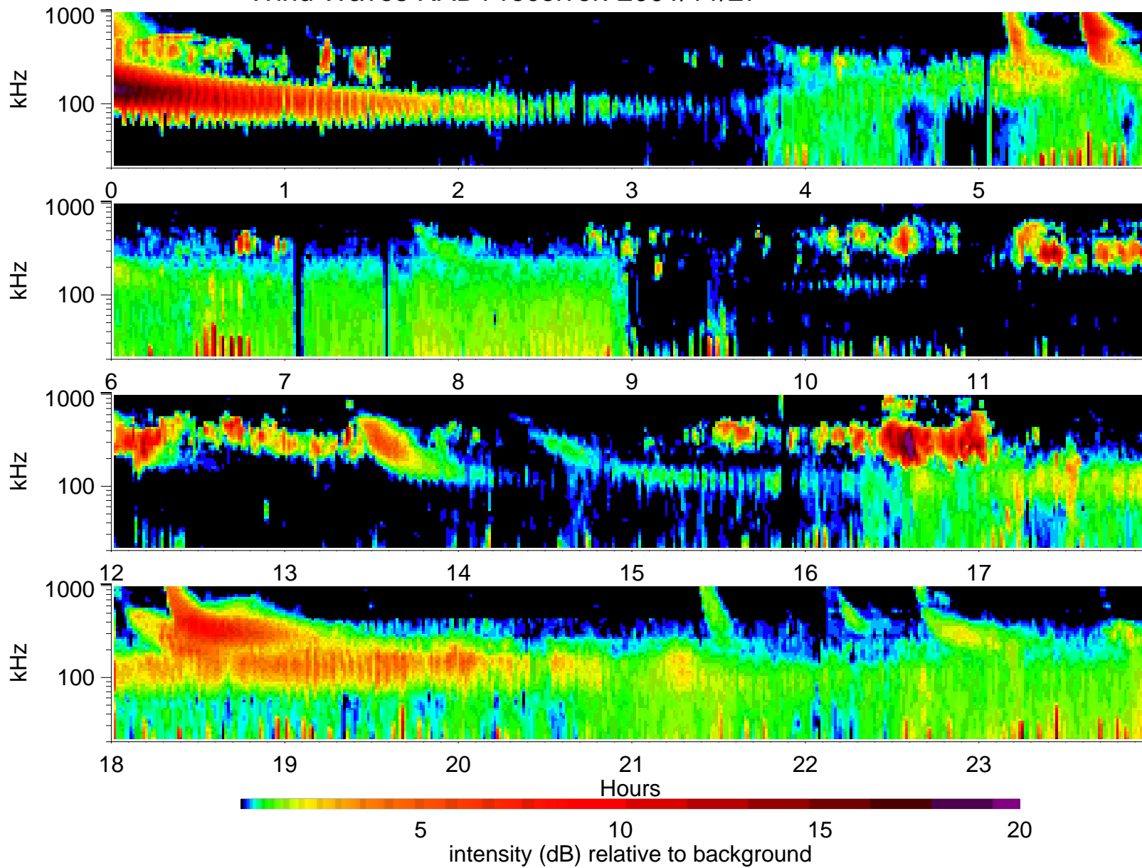
Wind Waves RAD1 receiver: 2001/11/27
