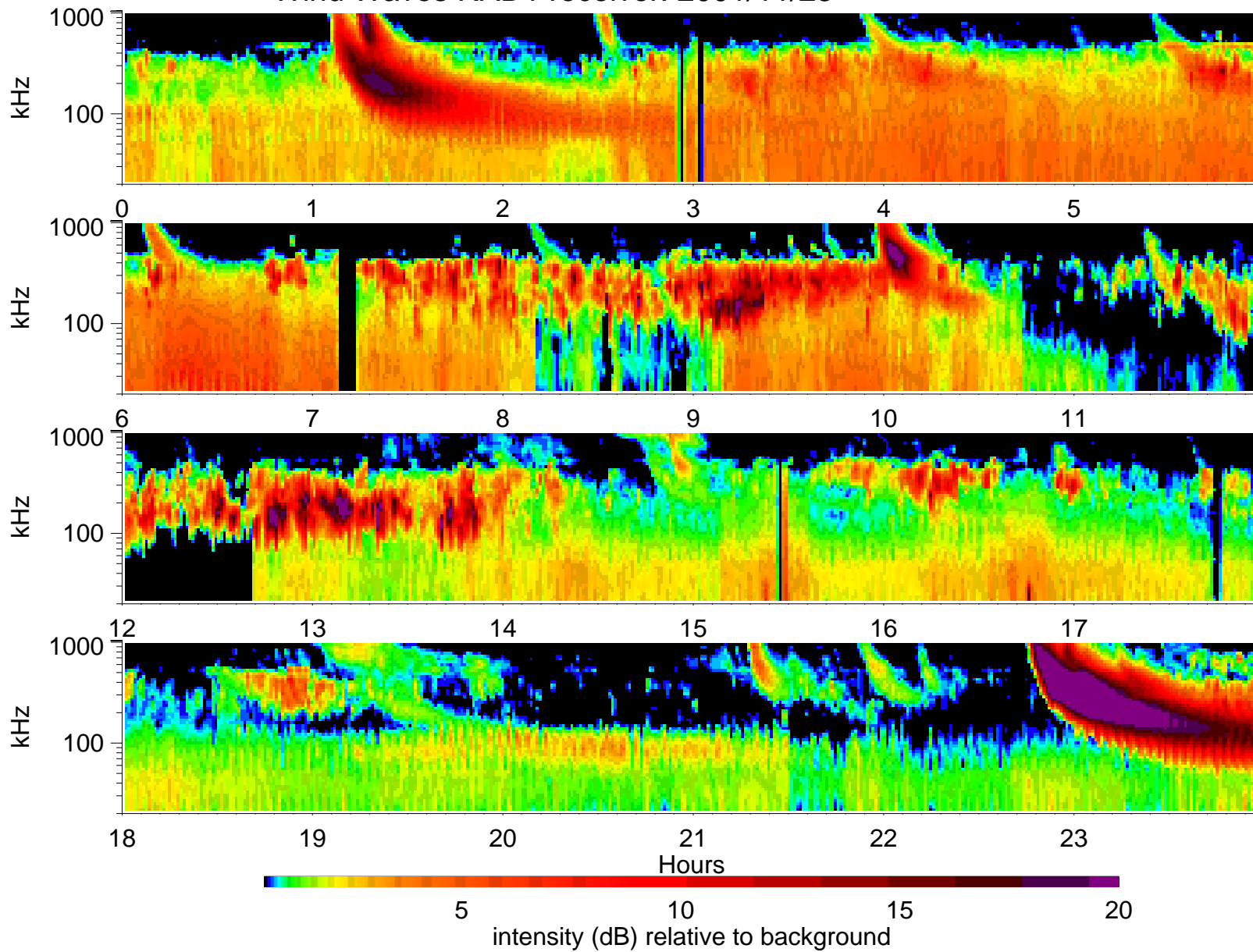
Wind Waves RAD1 receiver: 2001/11/25
