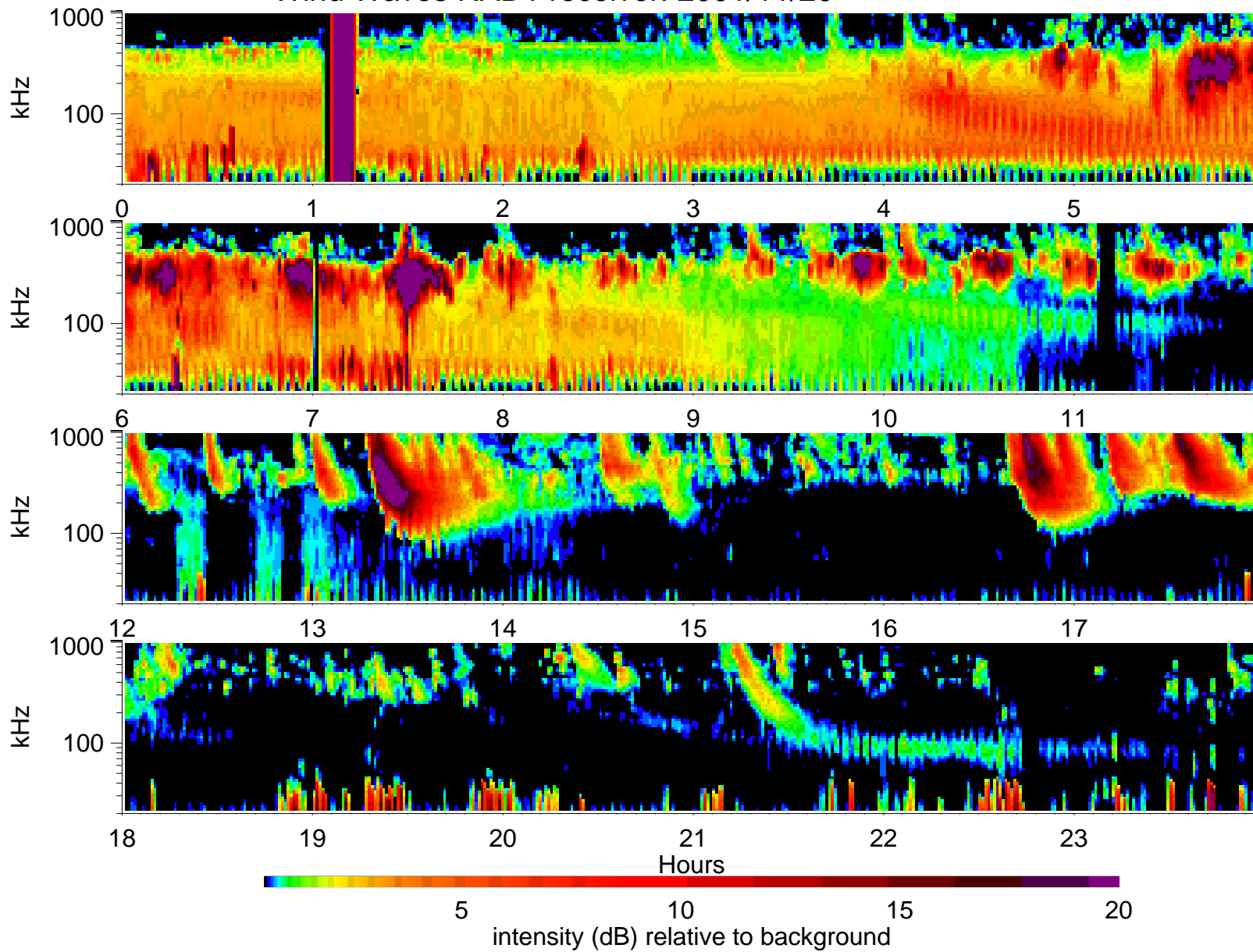
Wind Waves RAD1 receiver: 2001/11/20
