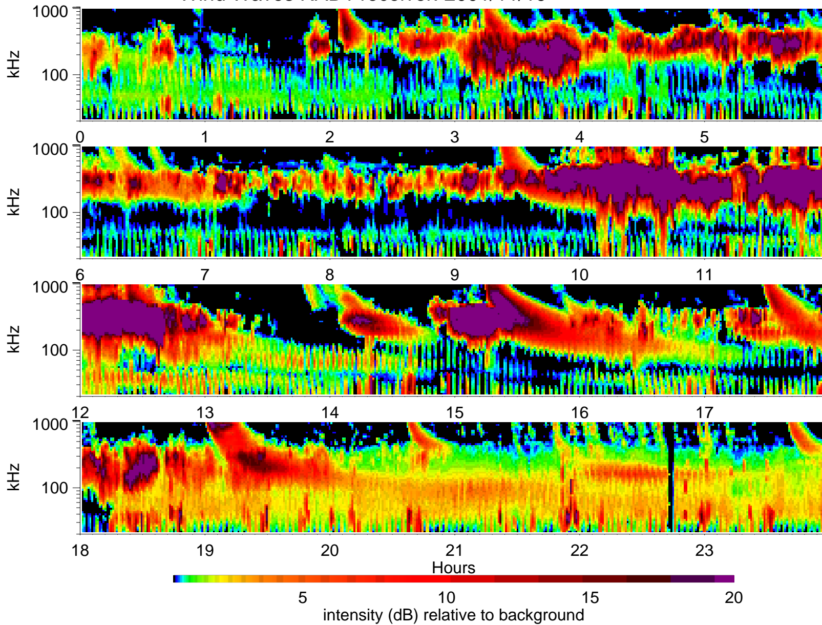
Wind Waves RAD1 receiver: 2001/11/19
