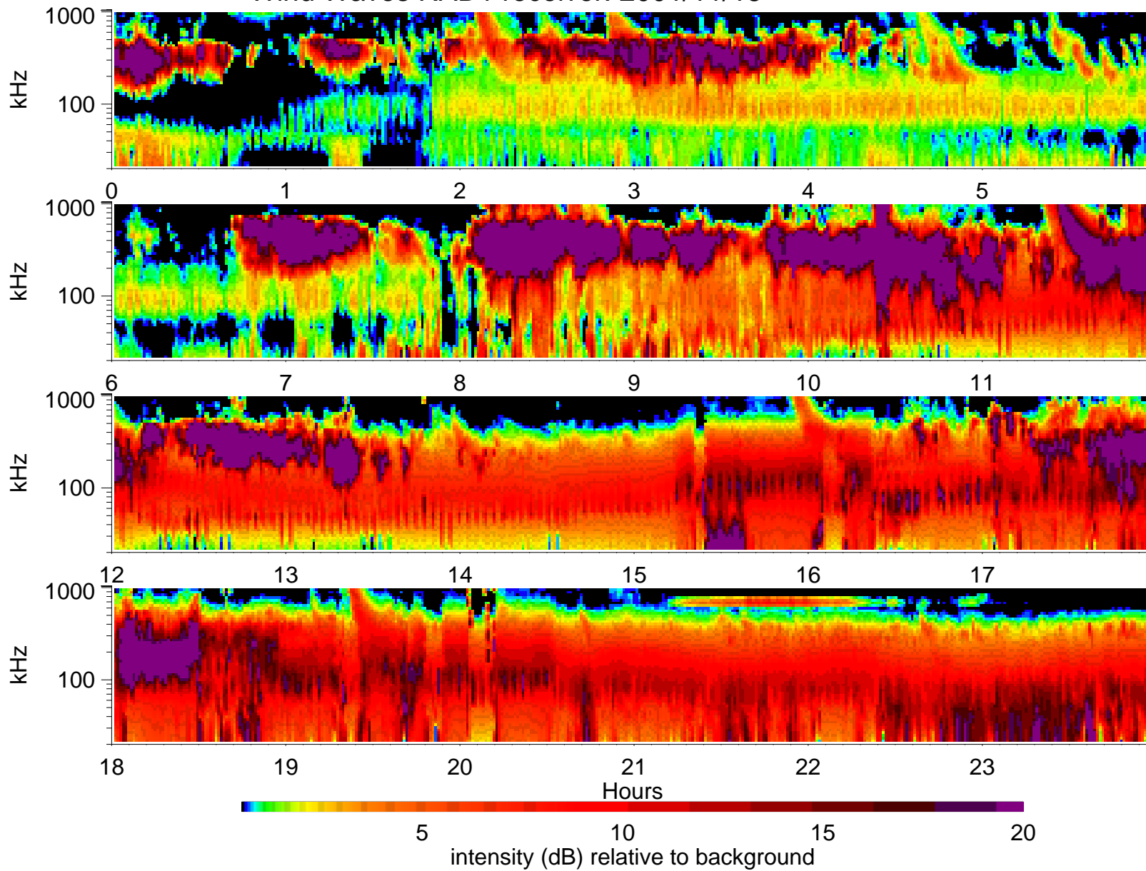
Wind Waves RAD1 receiver: 2001/11/15
