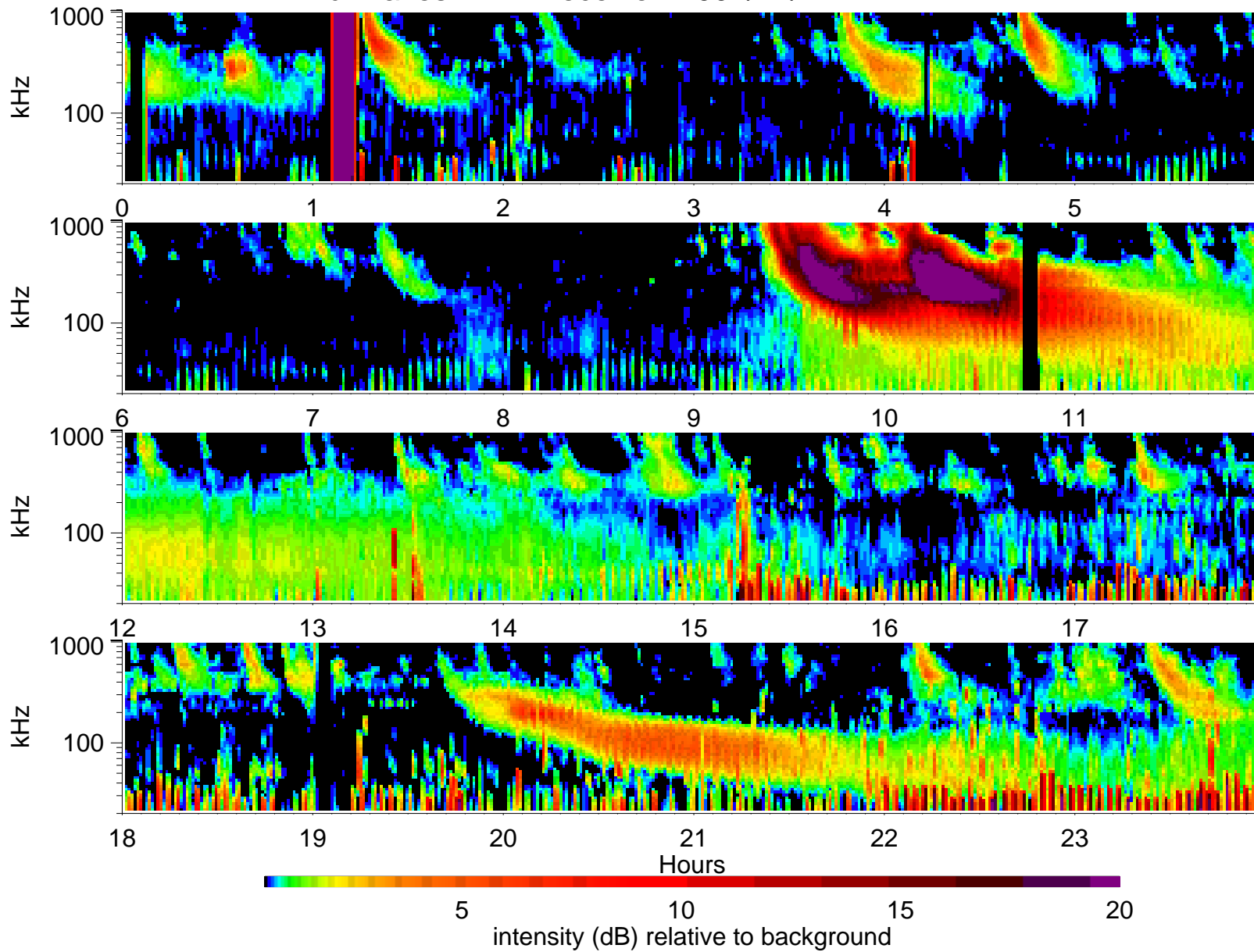
Wind Waves RAD1 receiver: 2001/11/12
