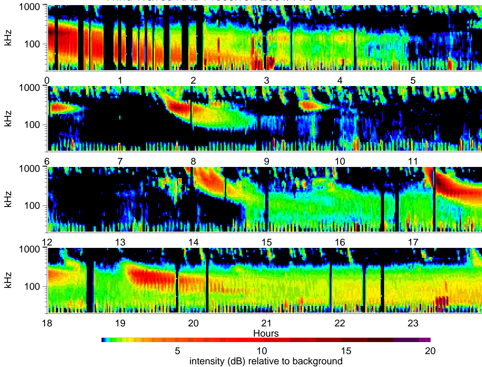
Wind Waves RAD1 receiver: 2001/11/3
