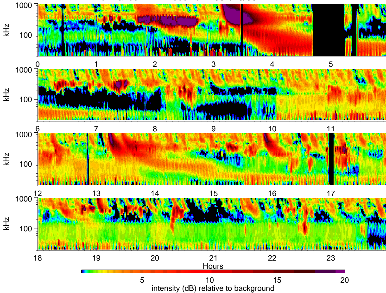
Wind Waves RAD1 receiver: 2001/10/30
