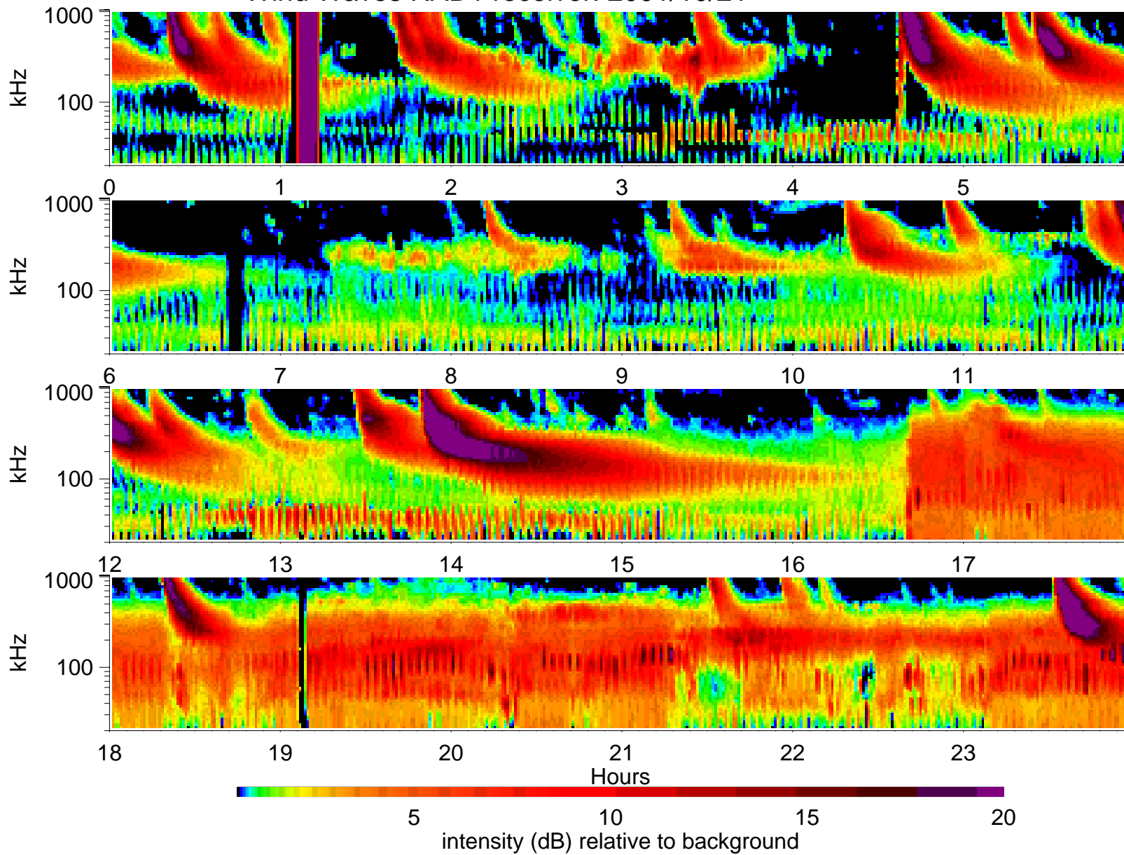
Wind Waves RAD1 receiver: 2001/10/21
