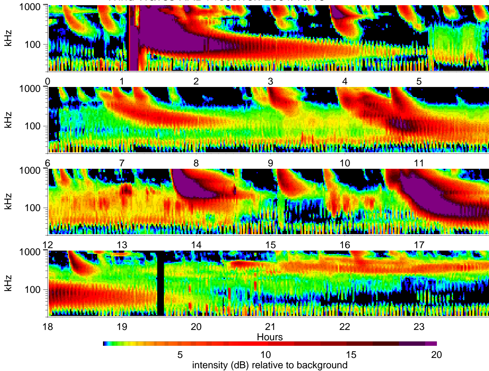
Wind Waves RAD1 receiver: 2001/10/19
