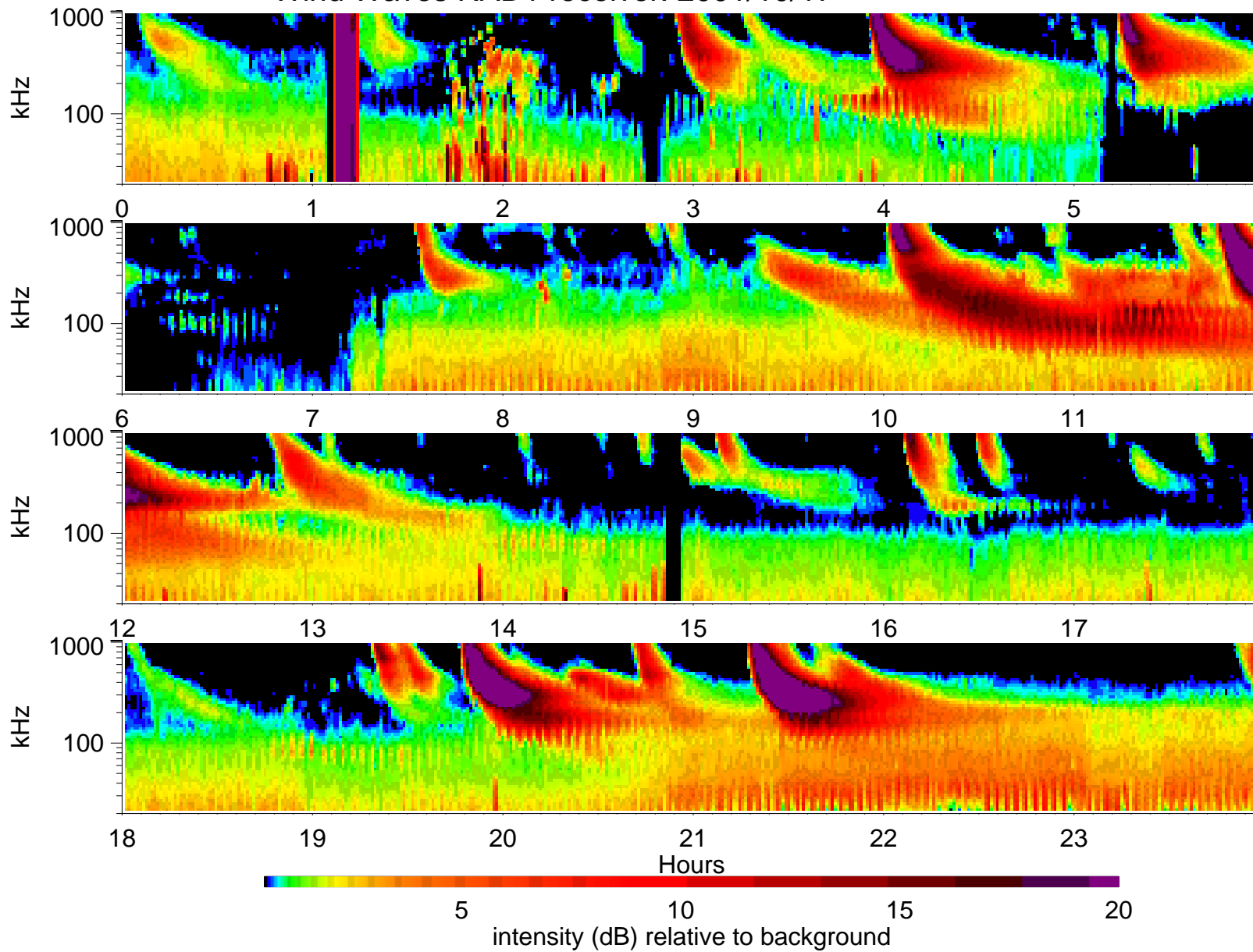
Wind Waves RAD1 receiver: 2001/10/17
