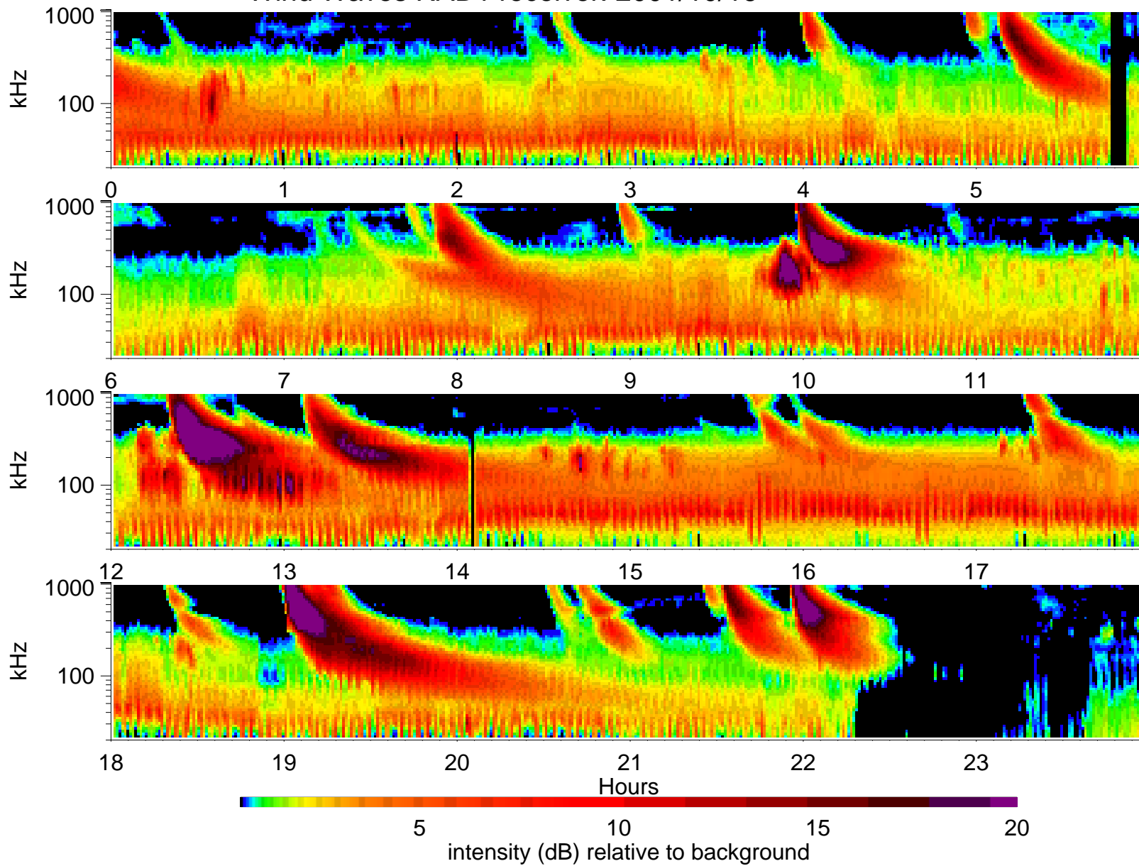
Wind Waves RAD1 receiver: 2001/10/16
