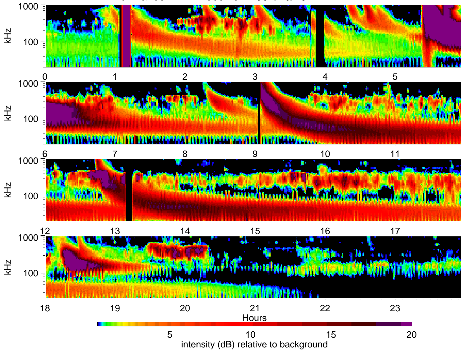
Wind Waves RAD1 receiver: 2001/10/13
