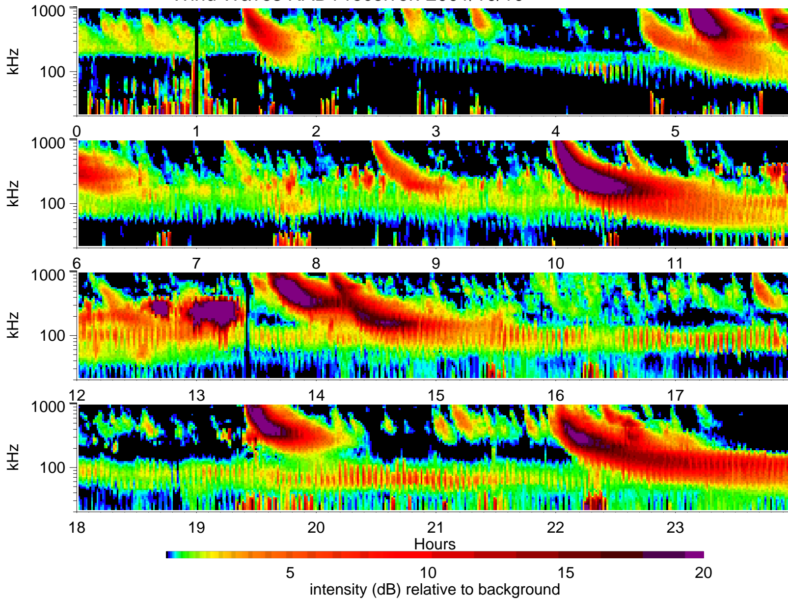
Wind Waves RAD1 receiver: 2001/10/10
