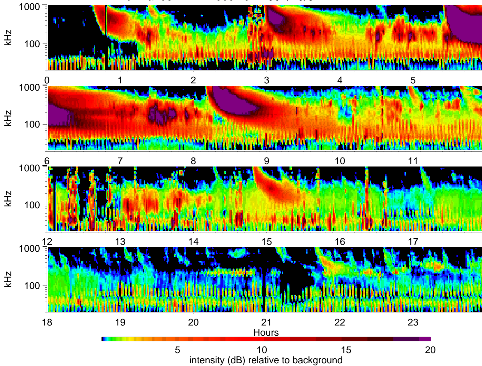
Wind Waves RAD1 receiver: 2001/10/8
