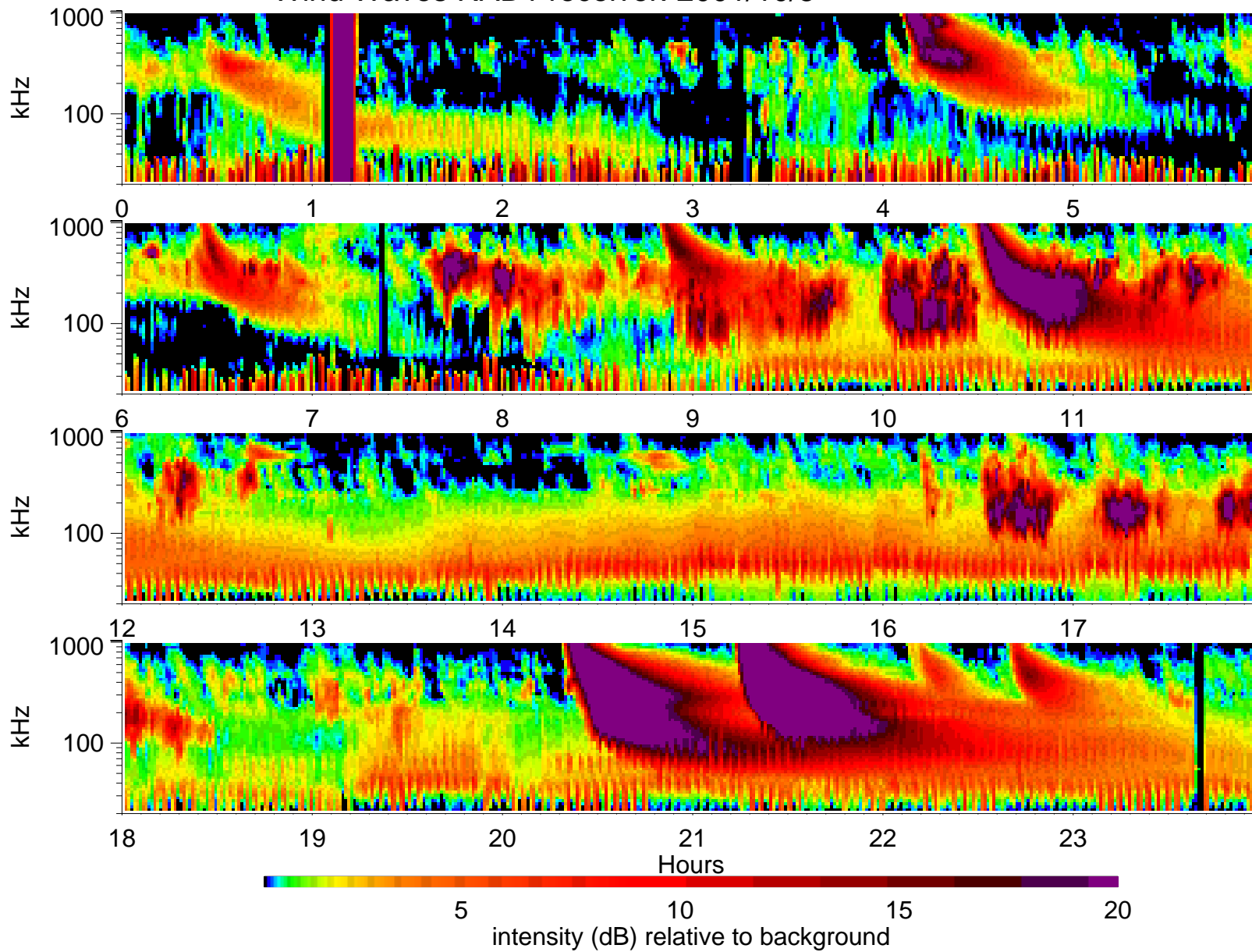
Wind Waves RAD1 receiver: 2001/10/5
