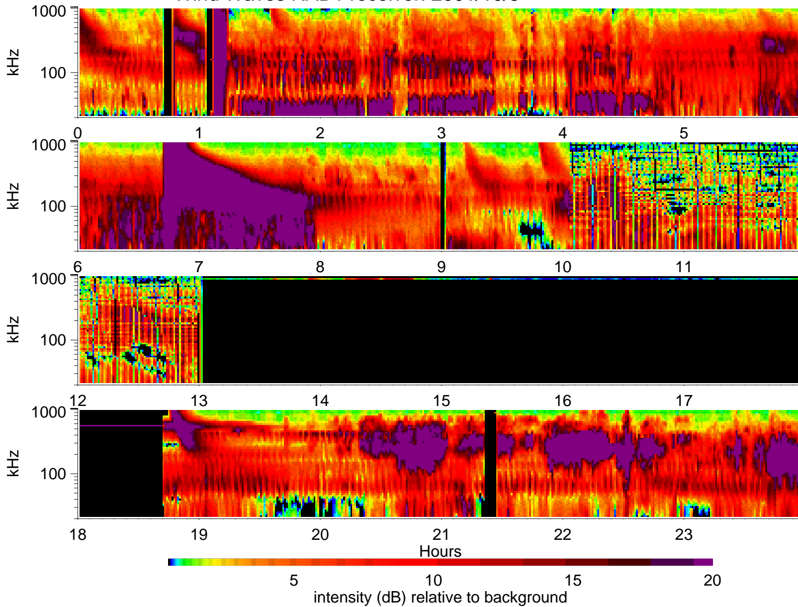
Wind Waves RAD1 receiver: 2001/10/3
