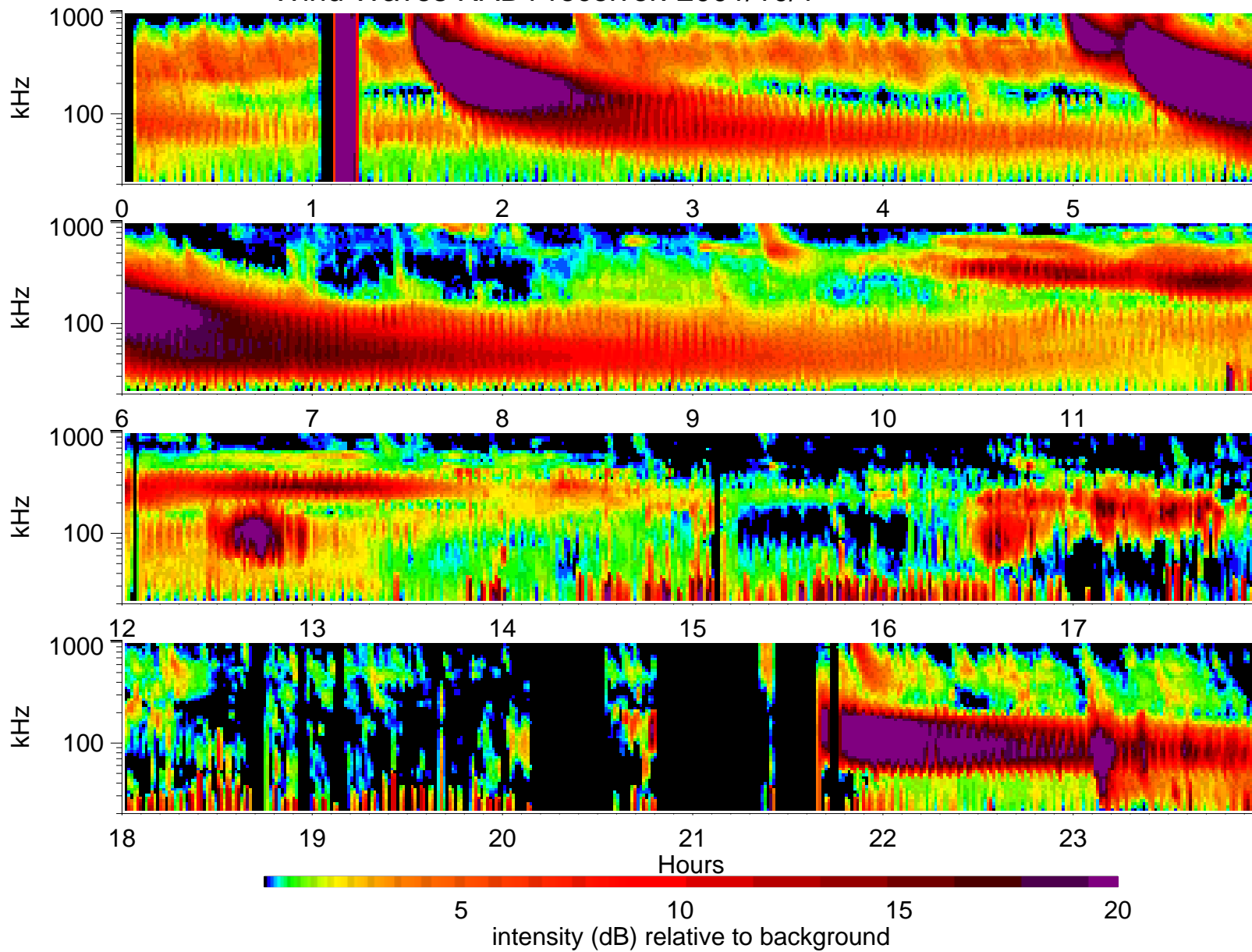
Wind Waves RAD1 receiver: 2001/10/1
