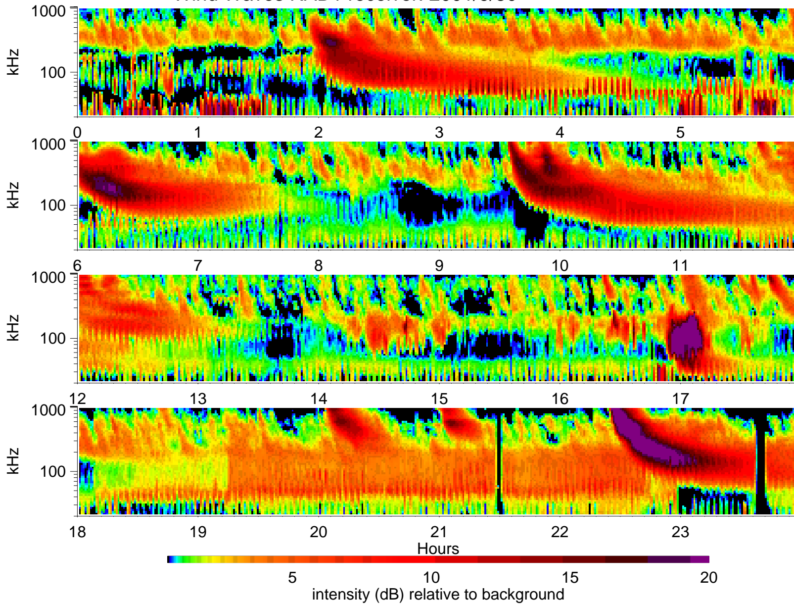
Wind Waves RAD1 receiver: 2001/9/30
