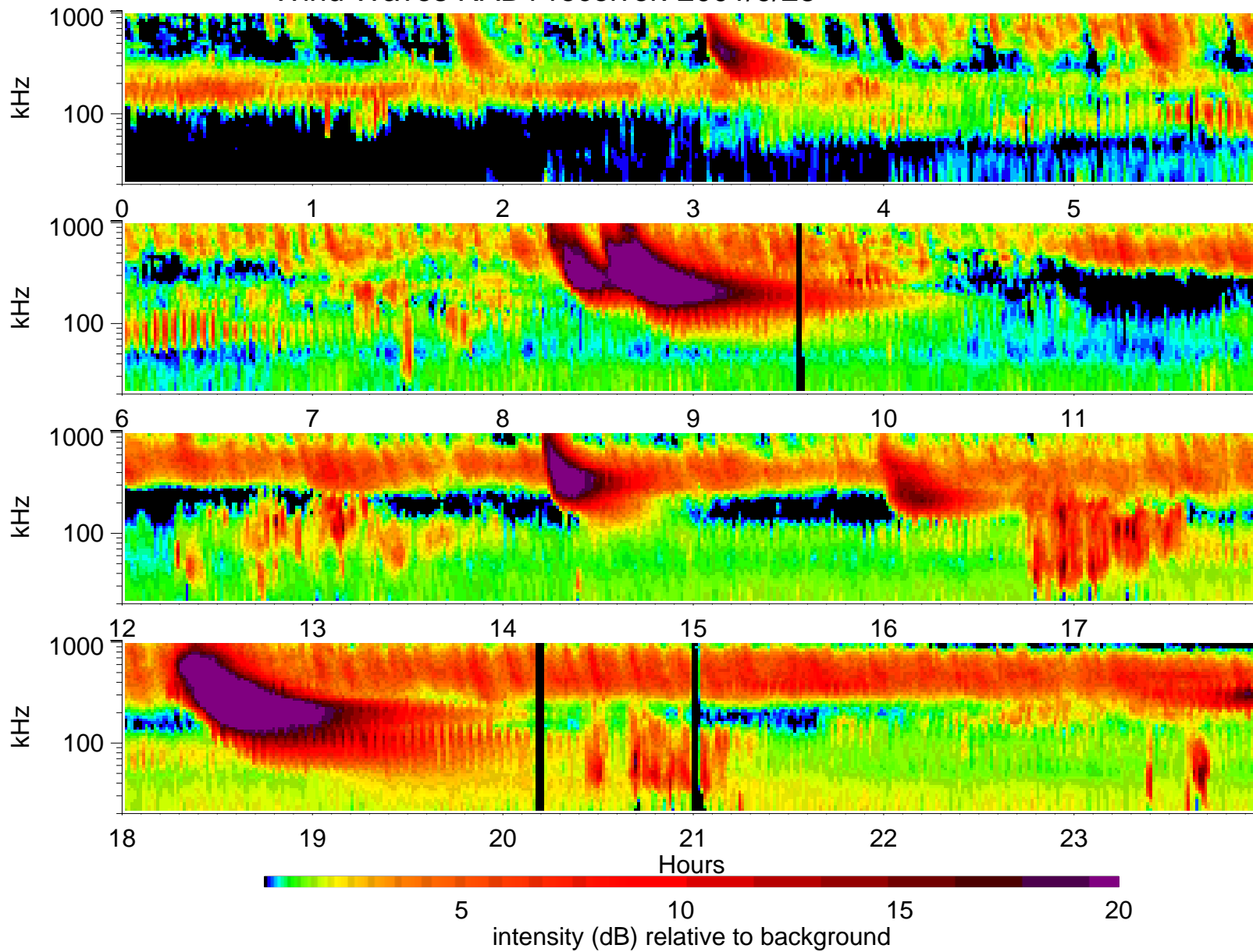
Wind Waves RAD1 receiver: 2001/9/28
