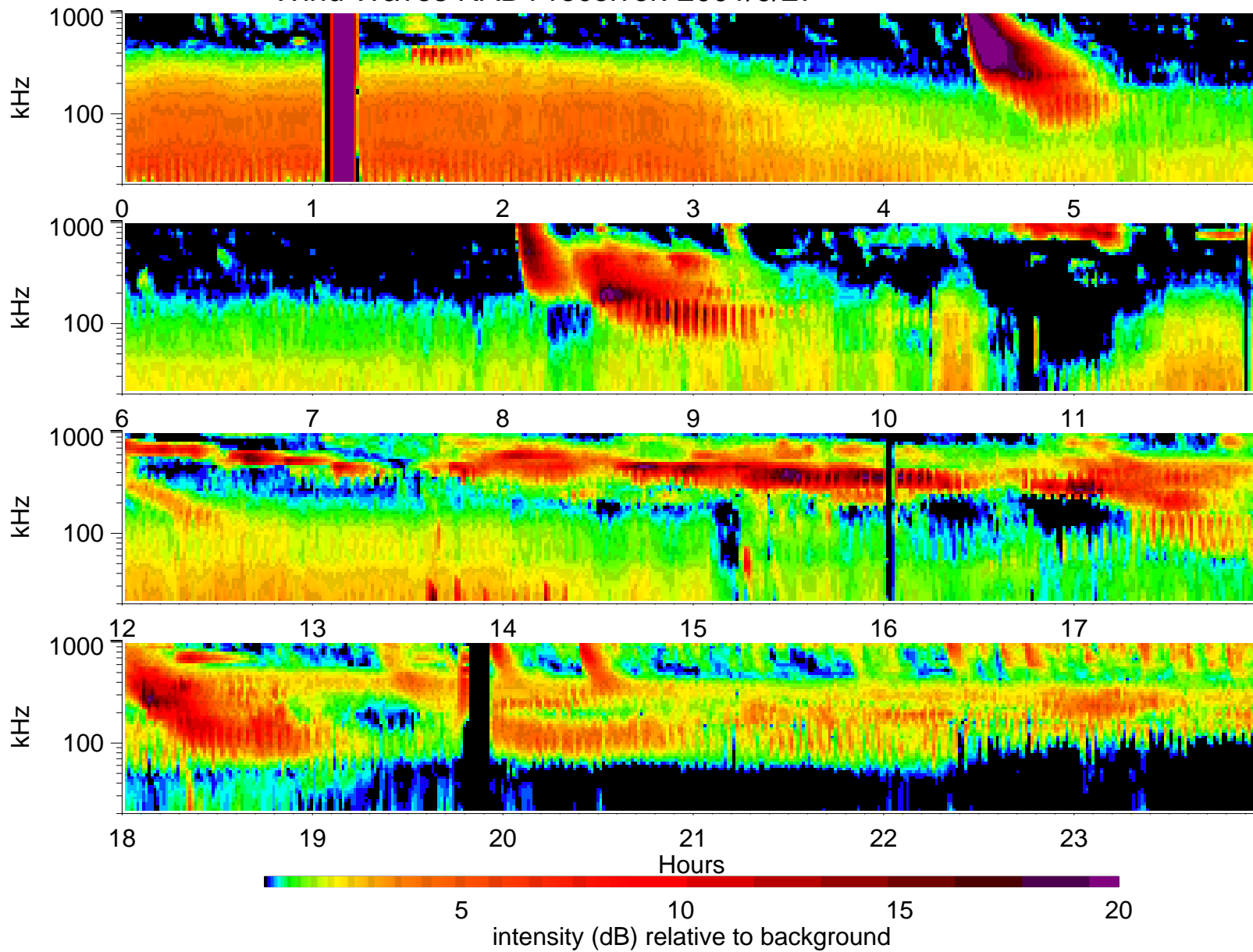
Wind Waves RAD1 receiver: 2001/9/27
