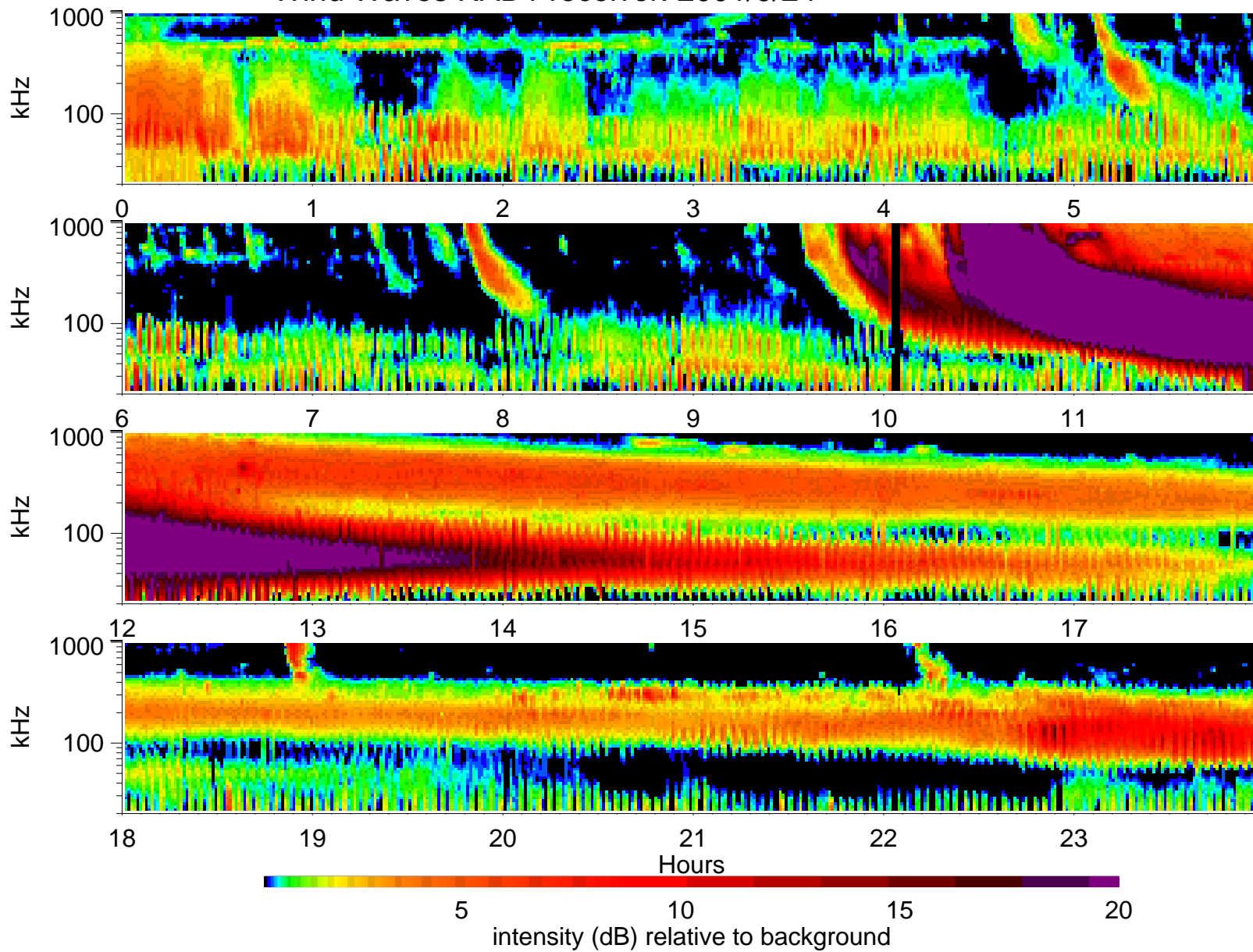
Wind Waves RAD1 receiver: 2001/9/24
