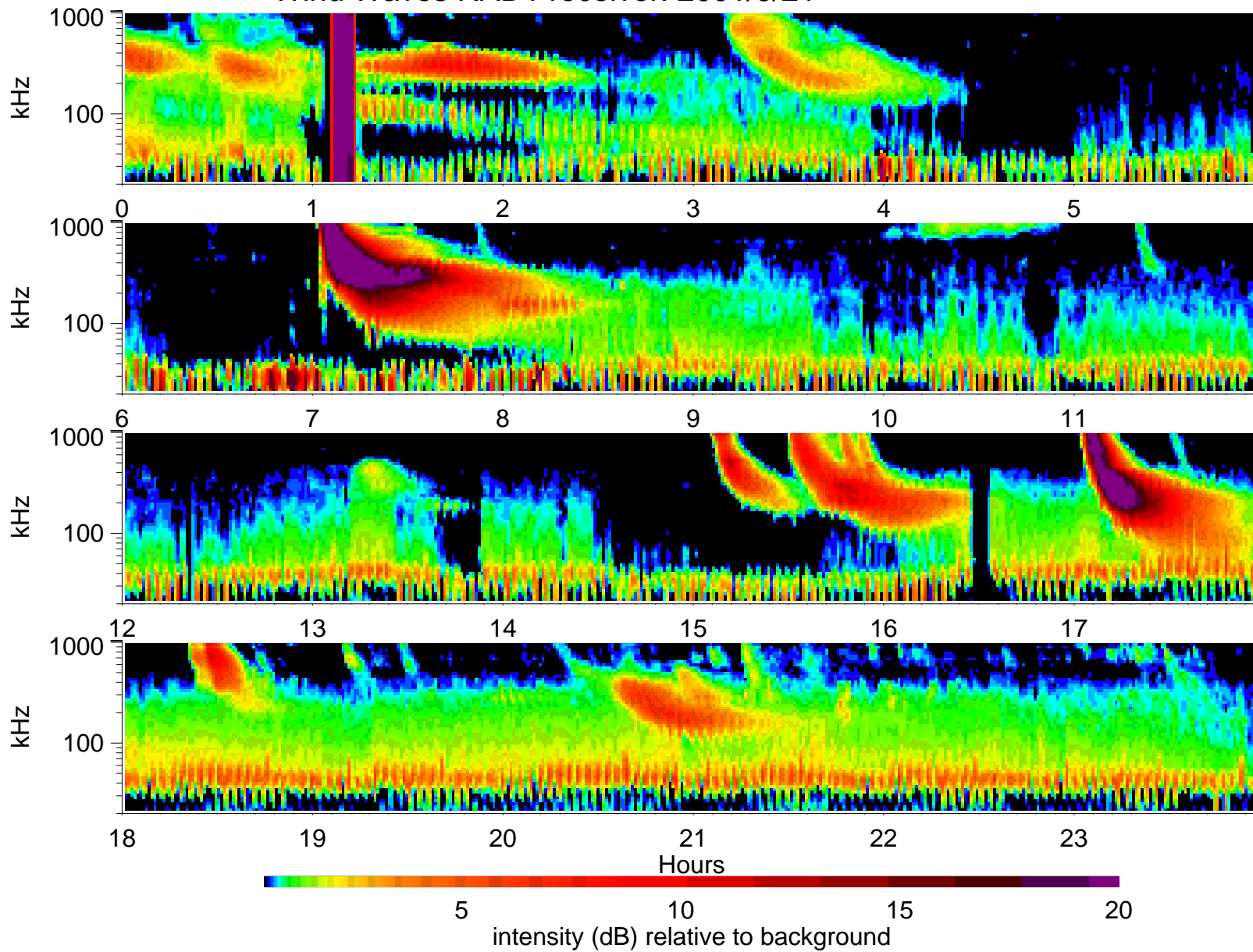
Wind Waves RAD1 receiver: 2001/9/21
