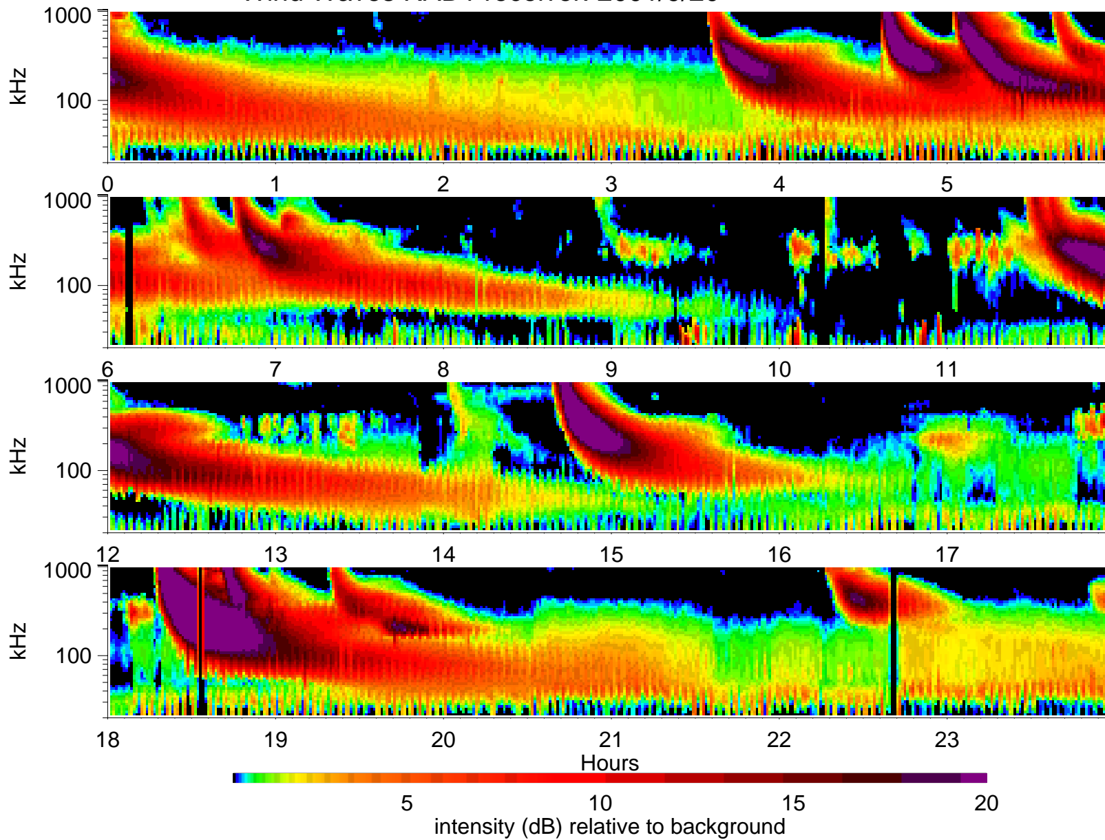
Wind Waves RAD1 receiver: 2001/9/20
