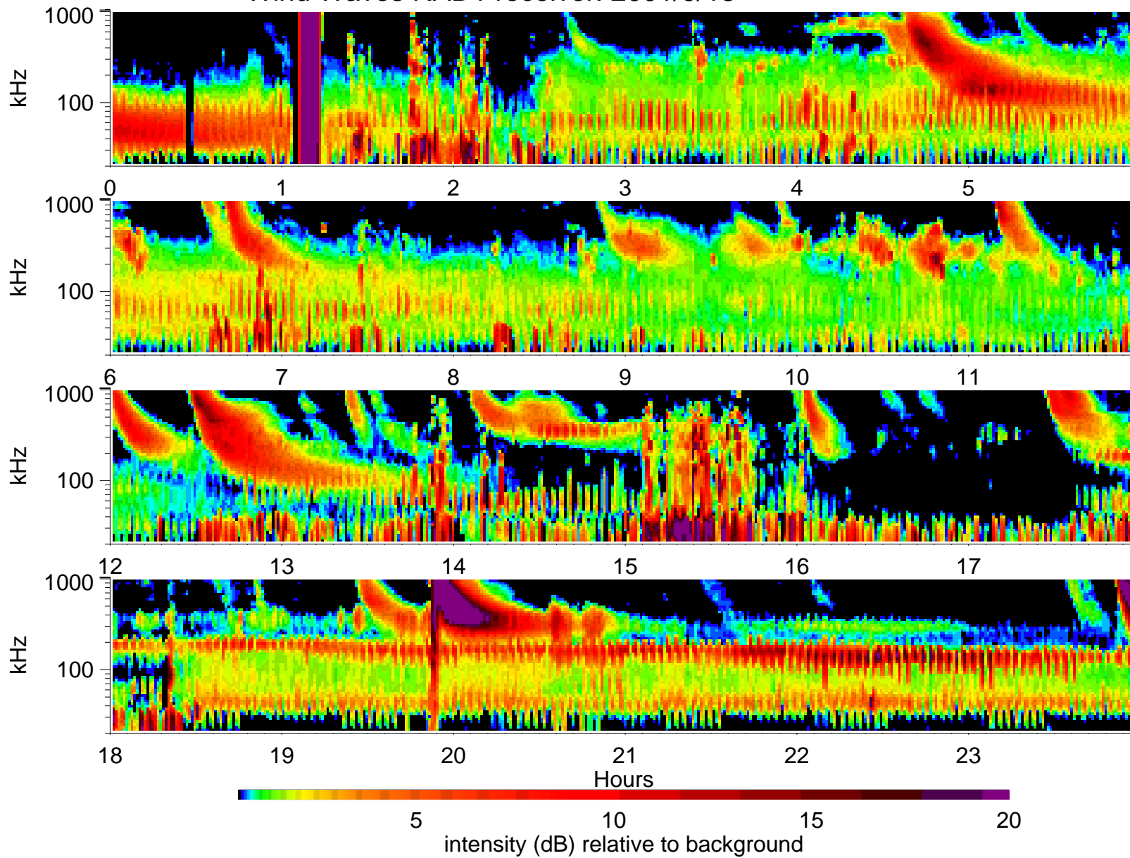
Wind Waves RAD1 receiver: 2001/9/13
