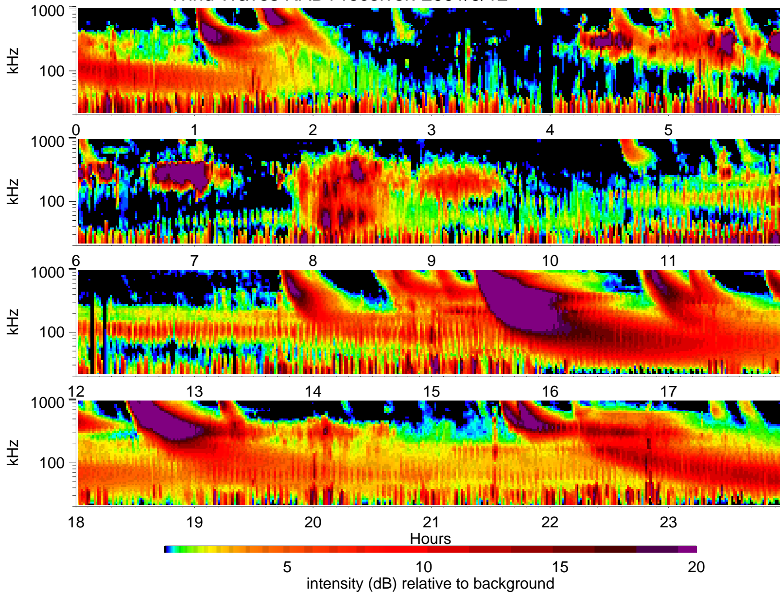
Wind Waves RAD1 receiver: 2001/9/12
