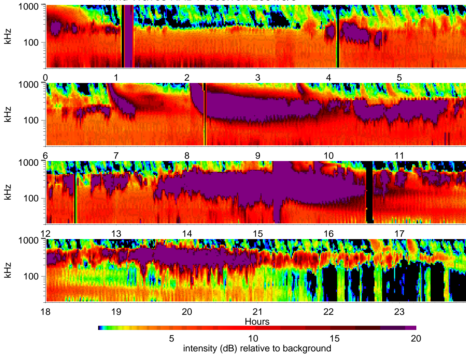
Wind Waves RAD1 receiver: 2001/9/9
