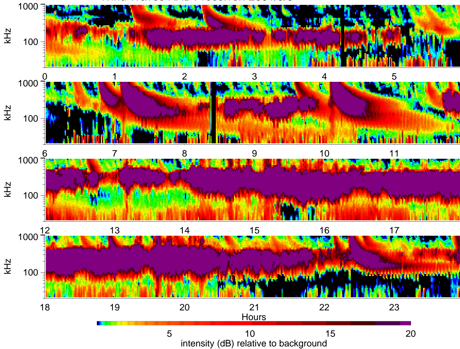
Wind Waves RAD1 receiver: 2001/9/8
