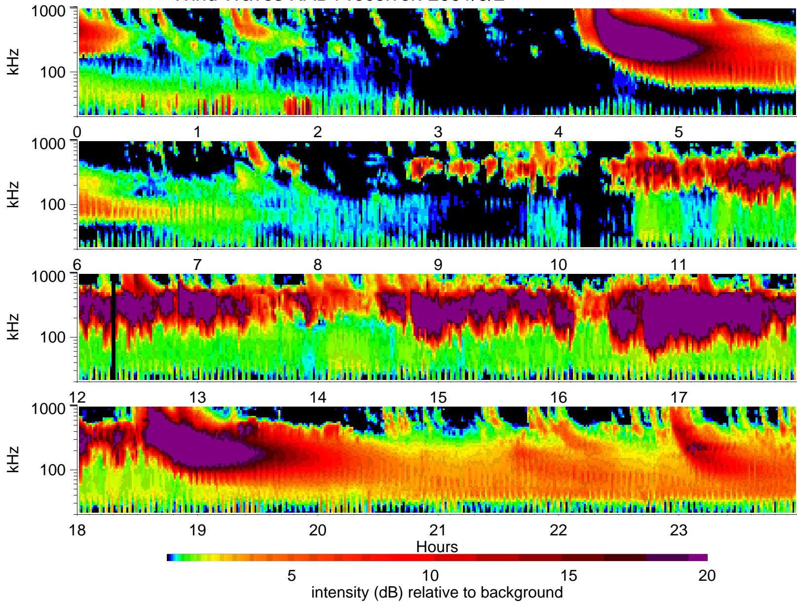
Wind Waves RAD1 receiver: 2001/9/2
