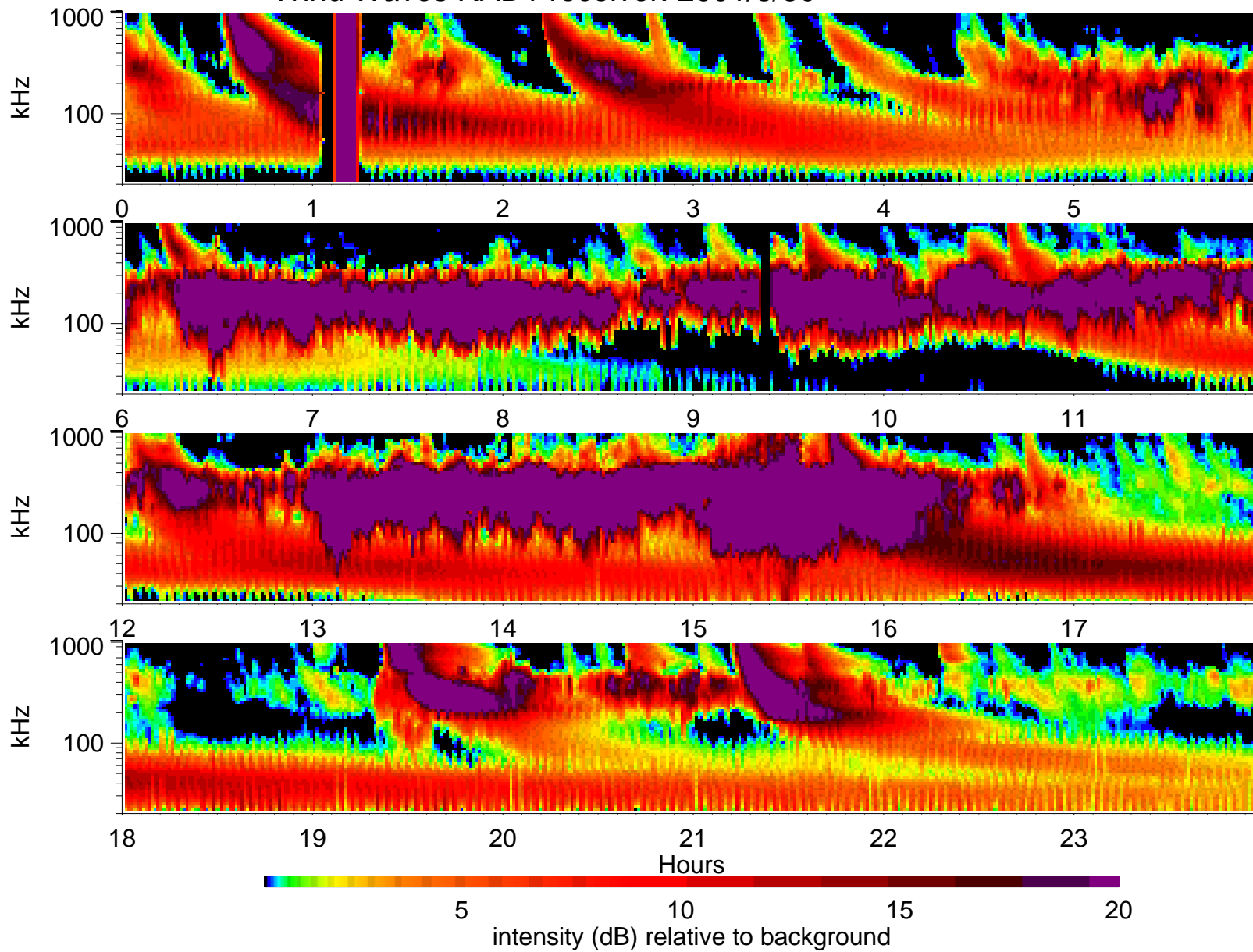
Wind Waves RAD1 receiver: 2001/8/30
