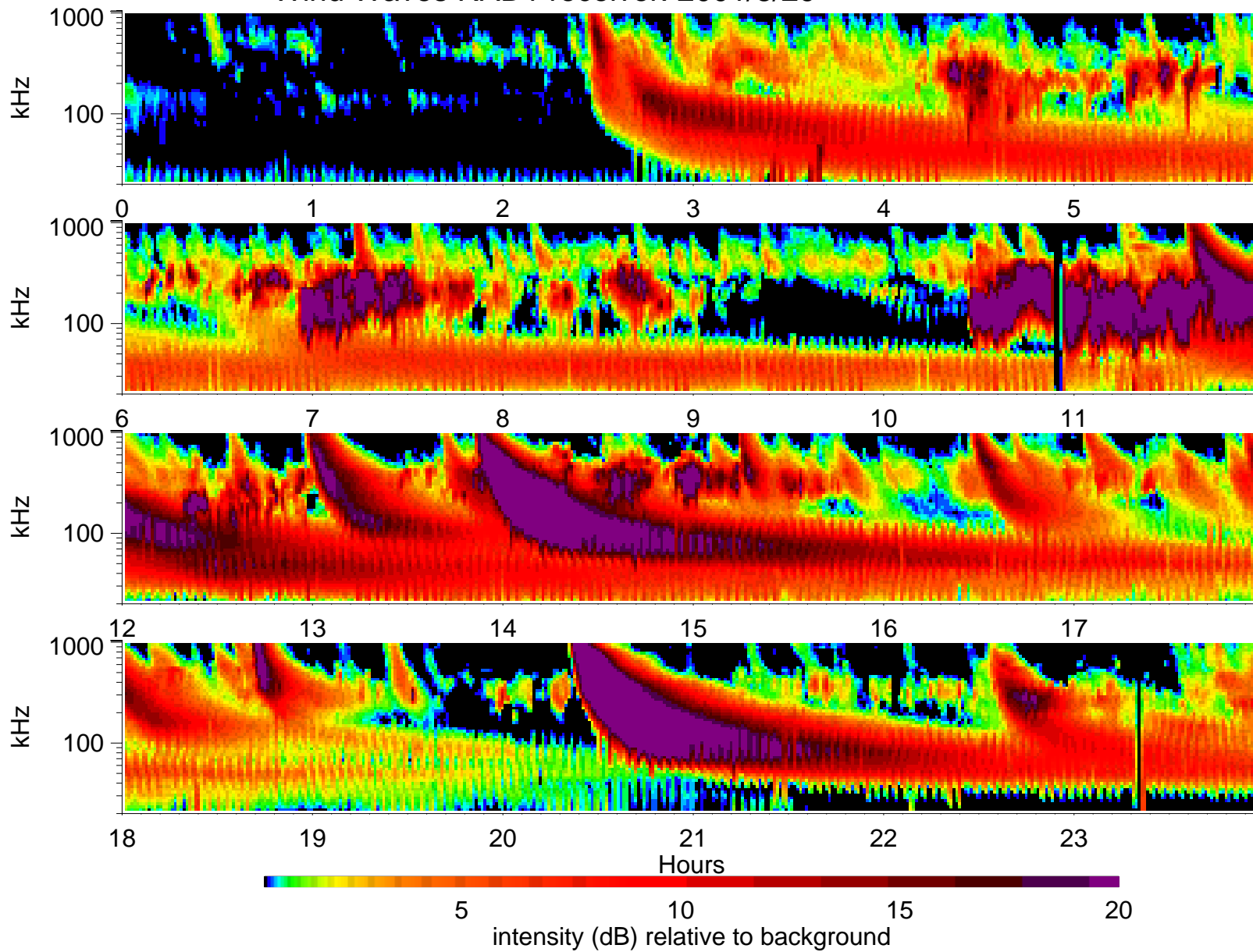
Wind Waves RAD1 receiver: 2001/8/29
