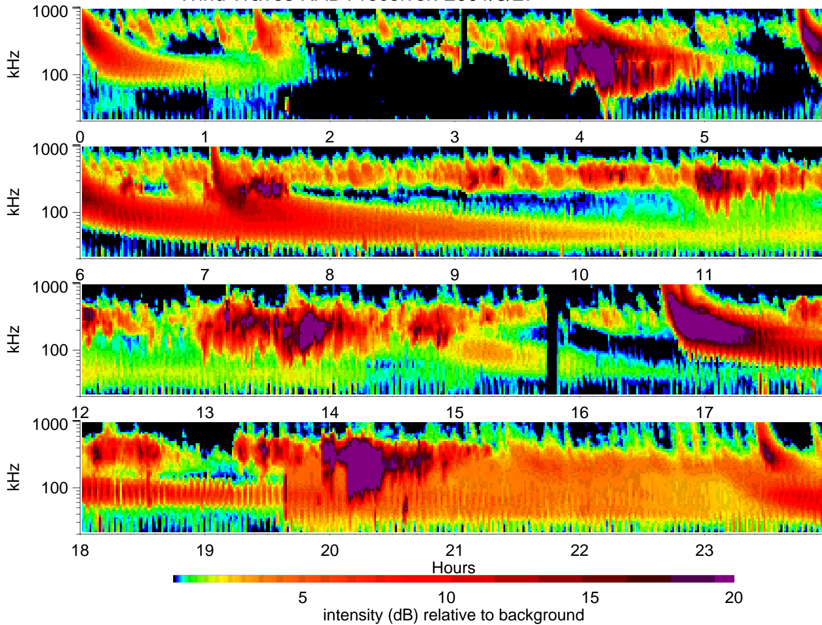
Wind Waves RAD1 receiver: 2001/8/27
