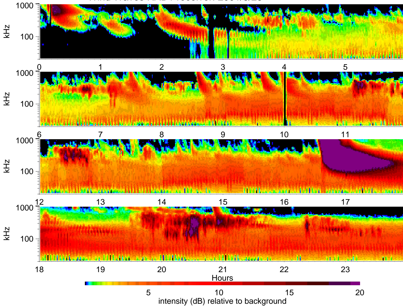
Wind Waves RAD1 receiver: 2001/8/25
