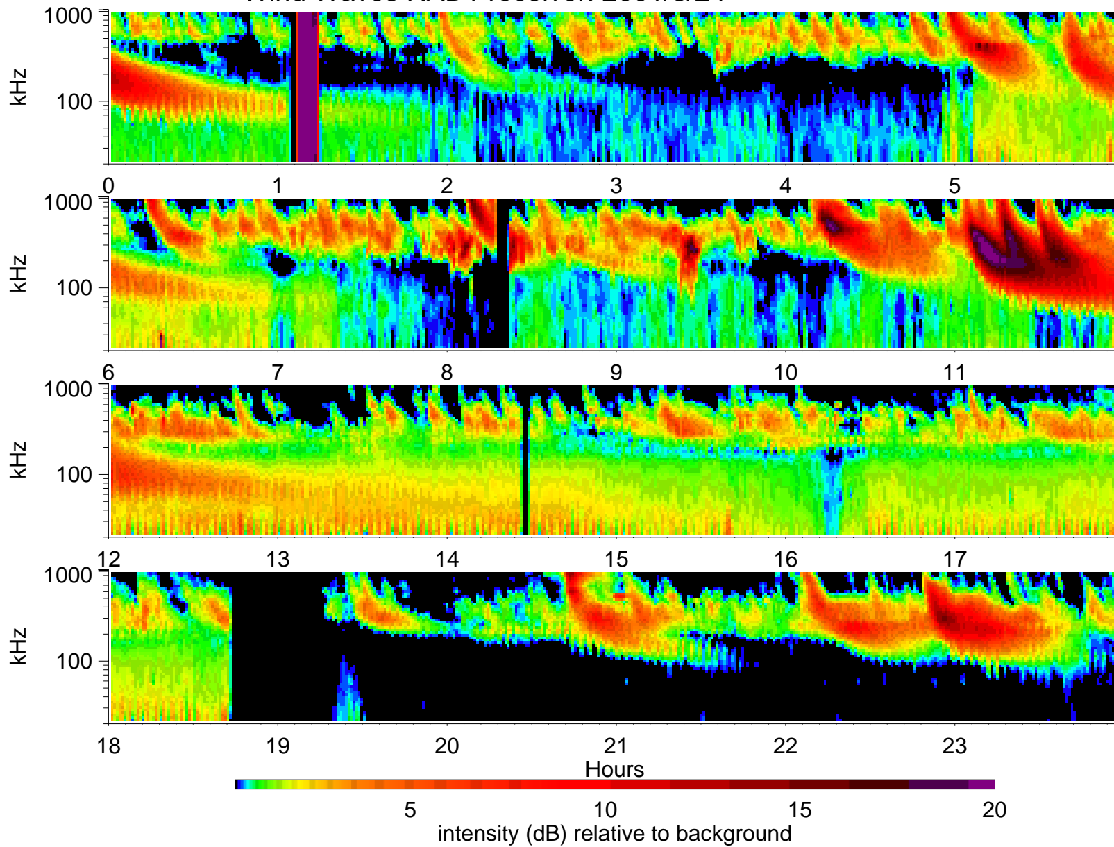
Wind Waves RAD1 receiver: 2001/8/24
