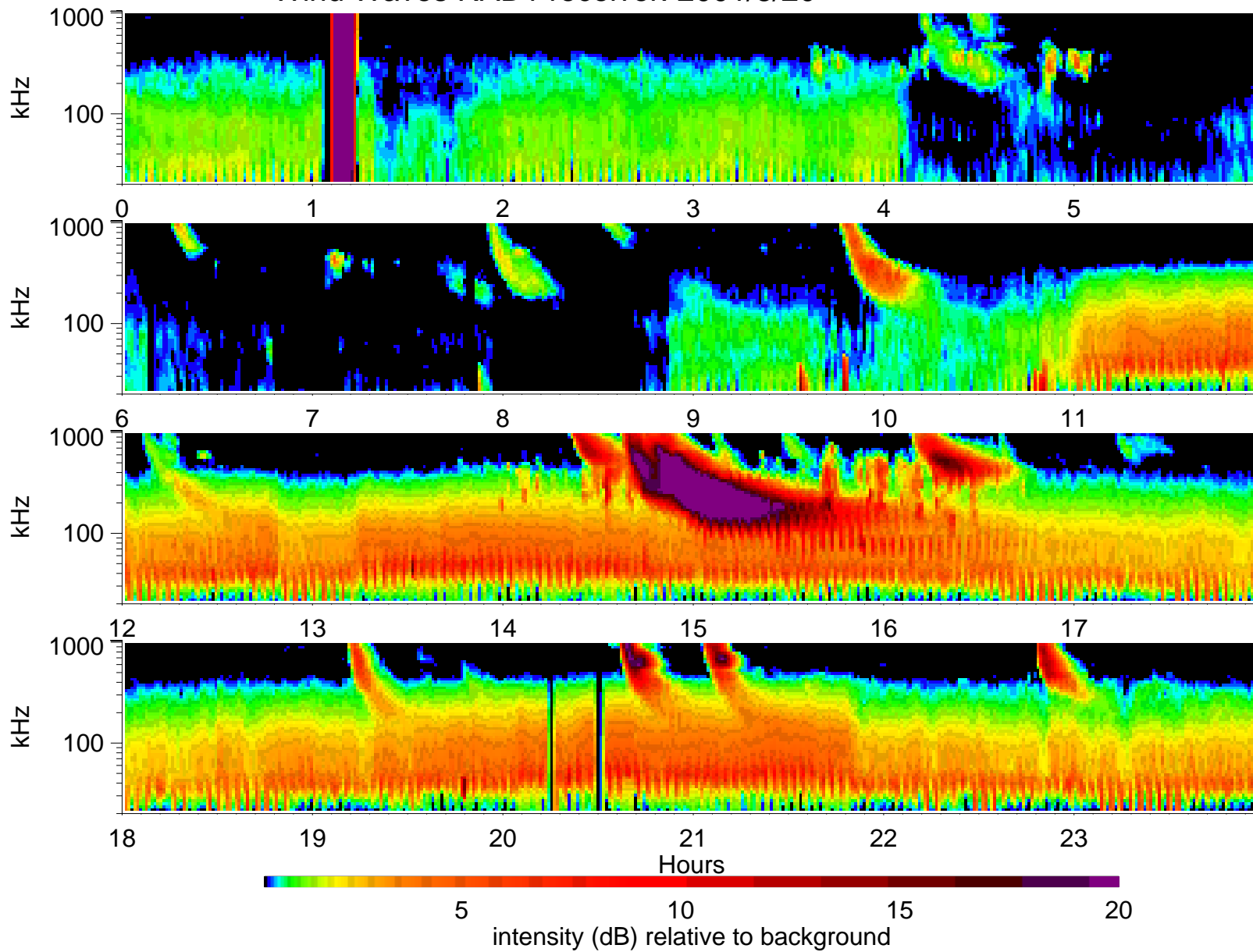
Wind Waves RAD1 receiver: 2001/8/20
