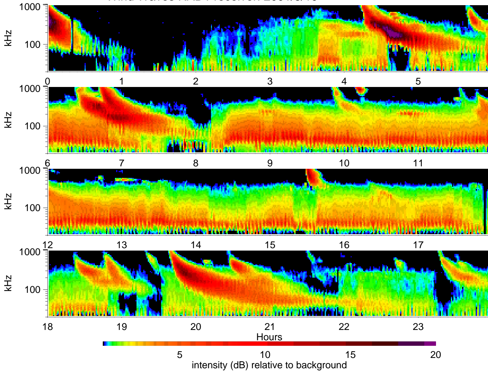
Wind Waves RAD1 receiver: 2001/8/19
