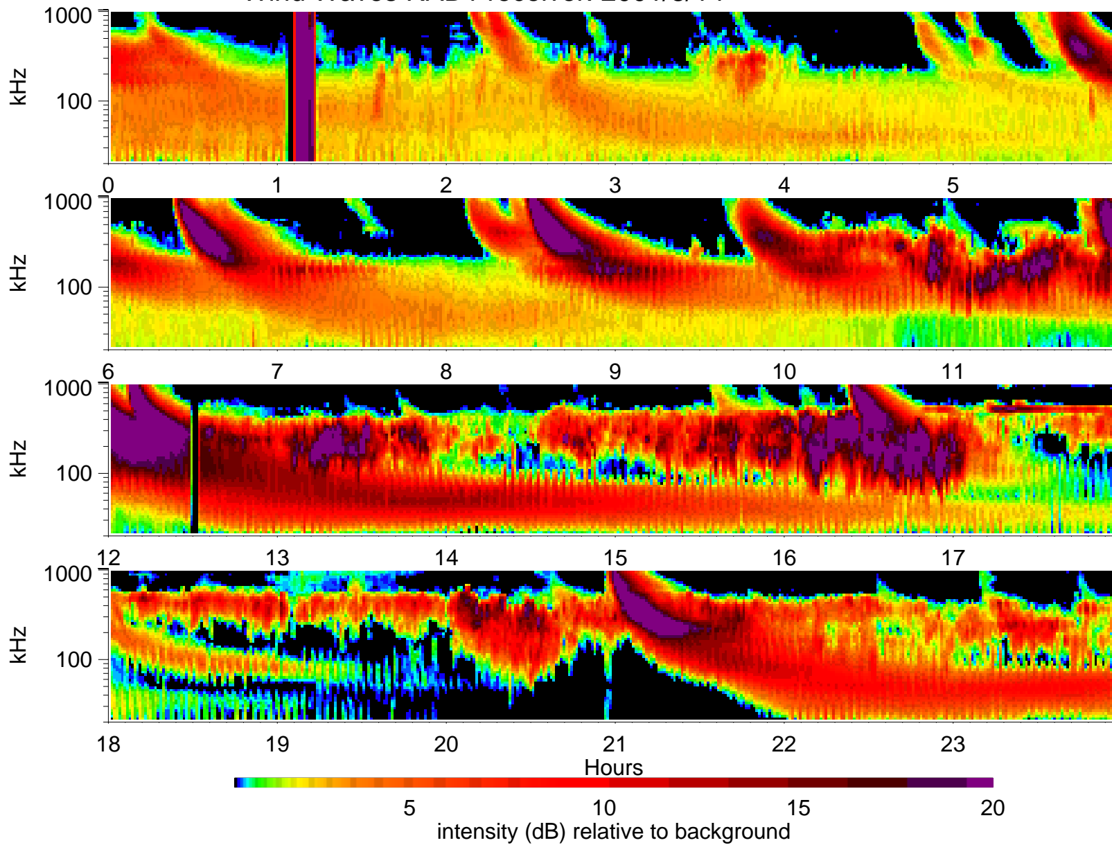
Wind Waves RAD1 receiver: 2001/8/14
