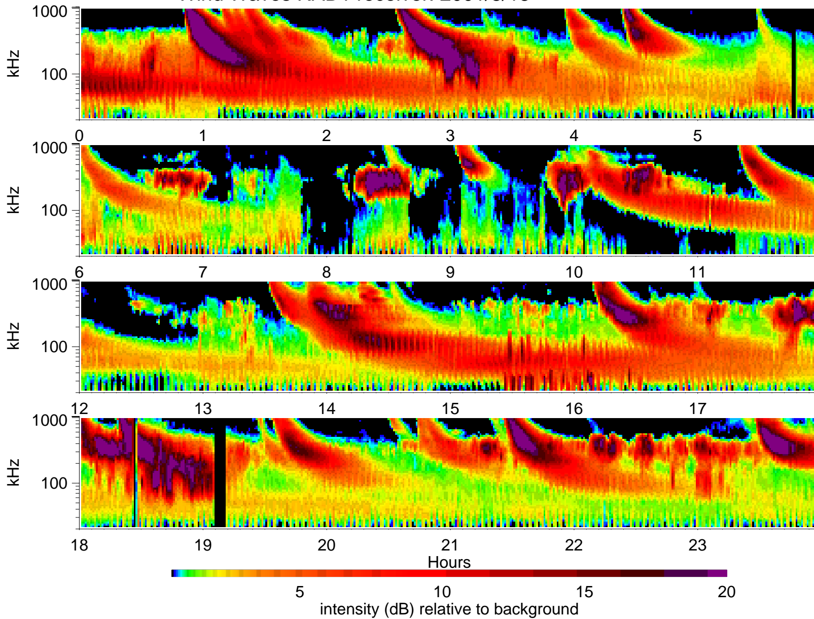
Wind Waves RAD1 receiver: 2001/8/13
