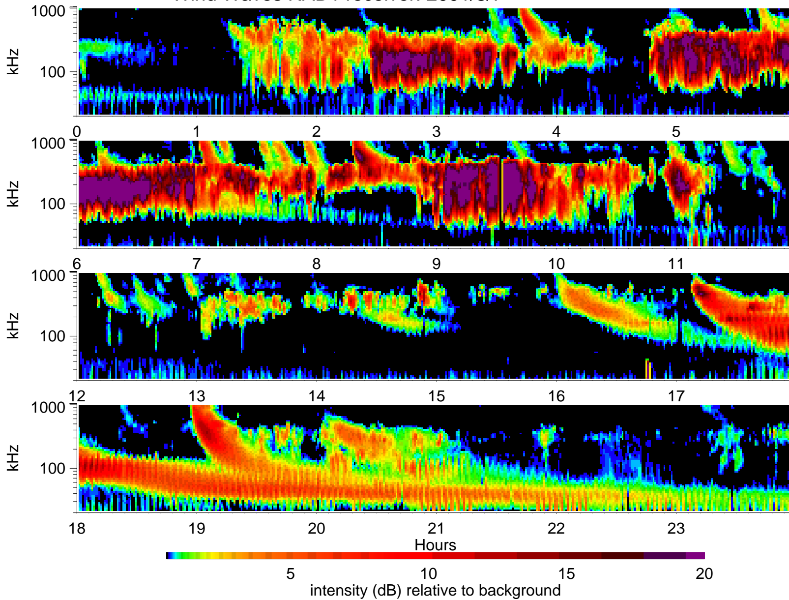
Wind Waves RAD1 receiver: 2001/8/7
