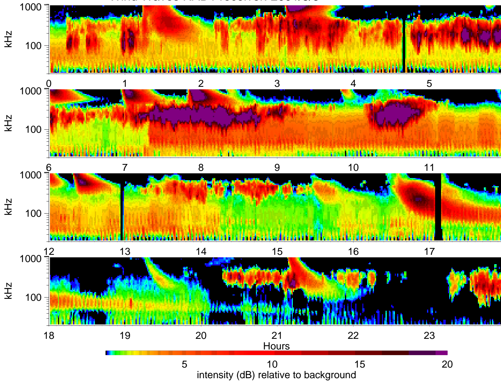
Wind Waves RAD1 receiver: 2001/8/3
