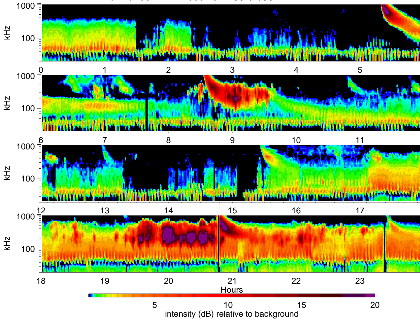
Wind Waves RAD1 receiver: 2001/7/30
