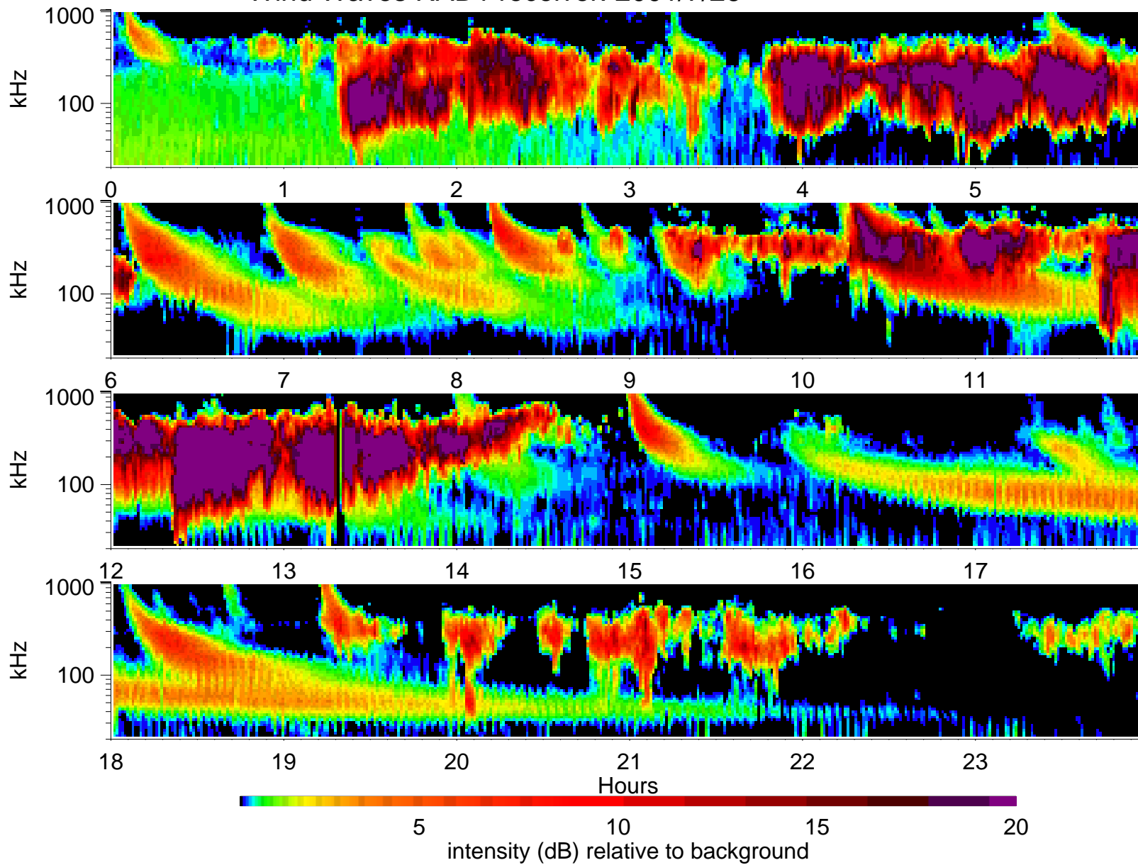
Wind Waves RAD1 receiver: 2001/7/26
