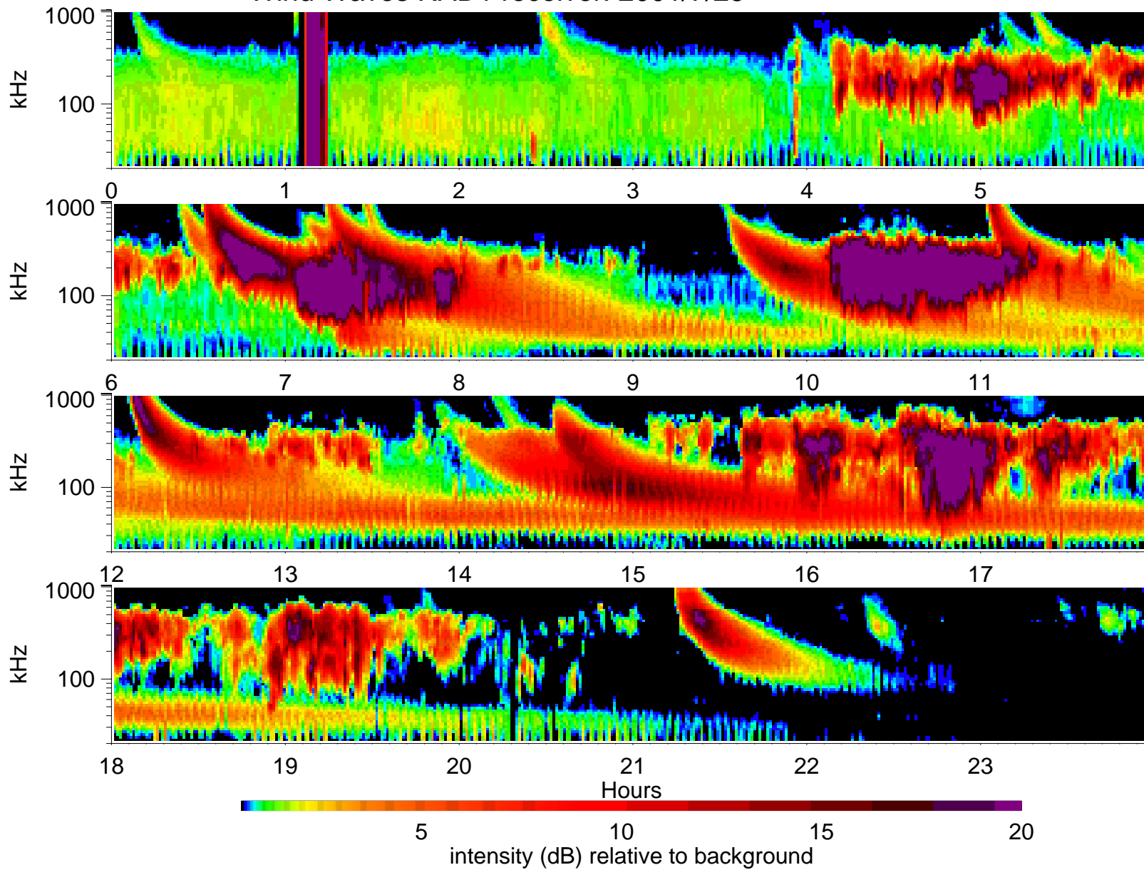
Wind Waves RAD1 receiver: 2001/7/25
