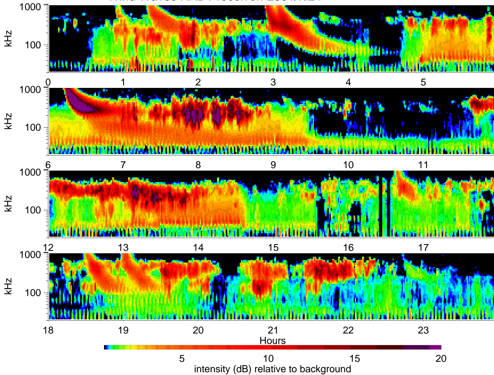
Wind Waves RAD1 receiver: 2001/7/24
